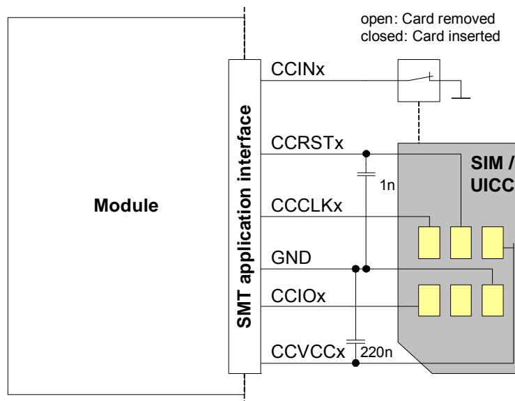
Figure 5: UICC/SIM/USIM interfaces
