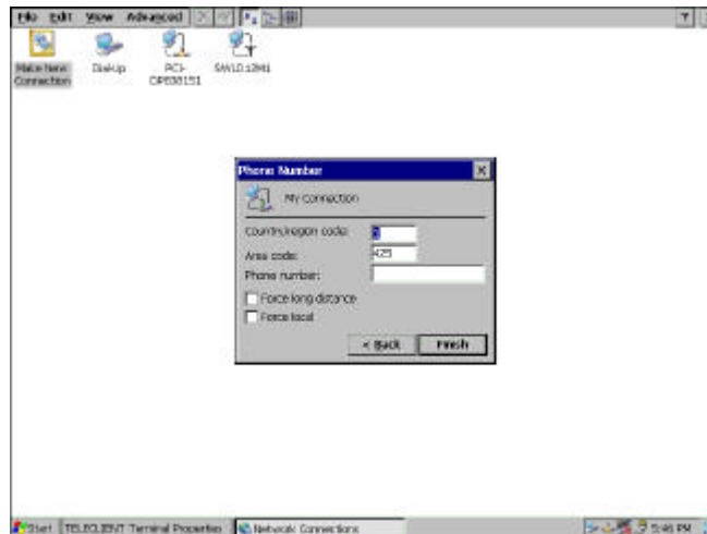
Figure 4.18 Dialing Properties
