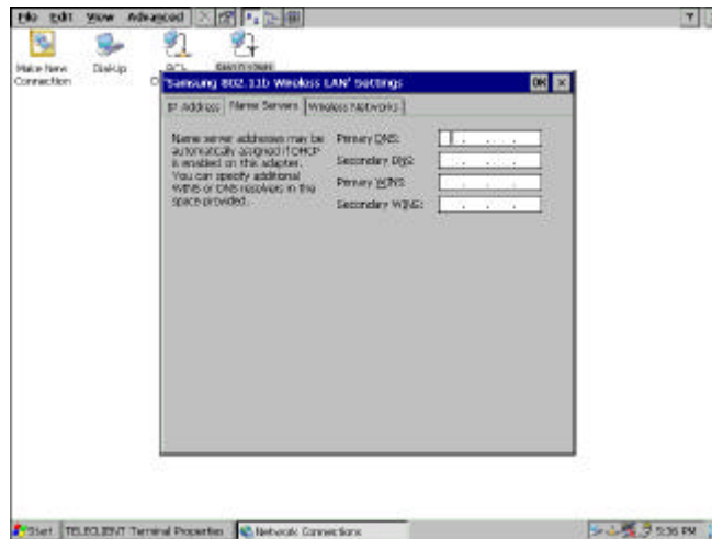
Figure 4.7 DNS/WINS Setting
