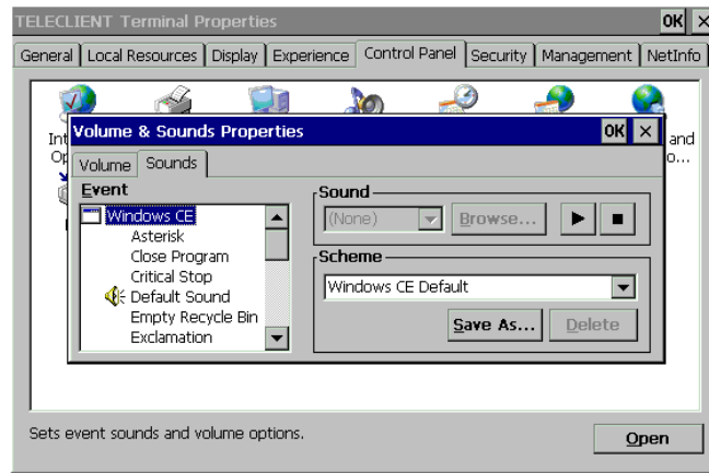
Figure 4.40 Sound Scheme
