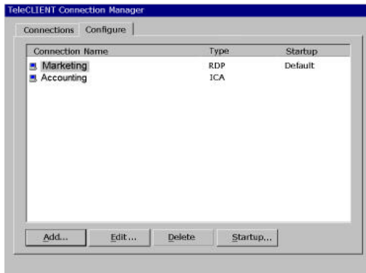
Figure 5.21 Configure Tab
