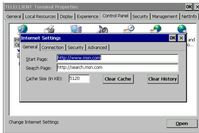
Figure 4.36 Internet Options
