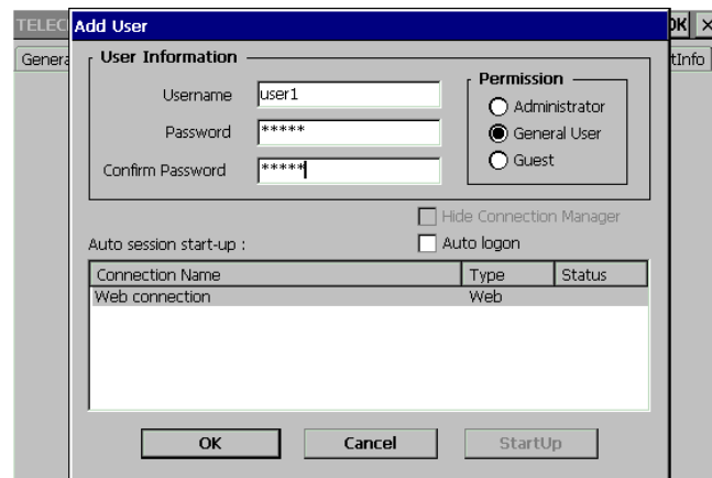
Figure 4.54 Security-Add User
