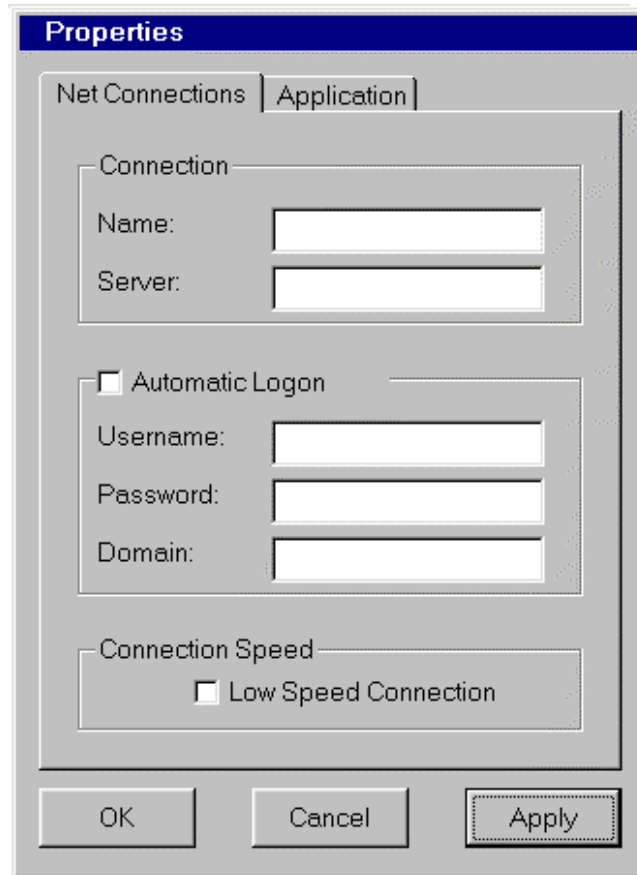
Figure 5.22 Properties Window
