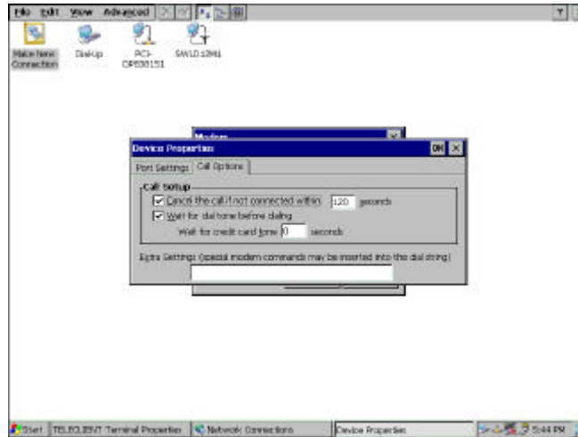
Figure 4.14 Dialing Options
