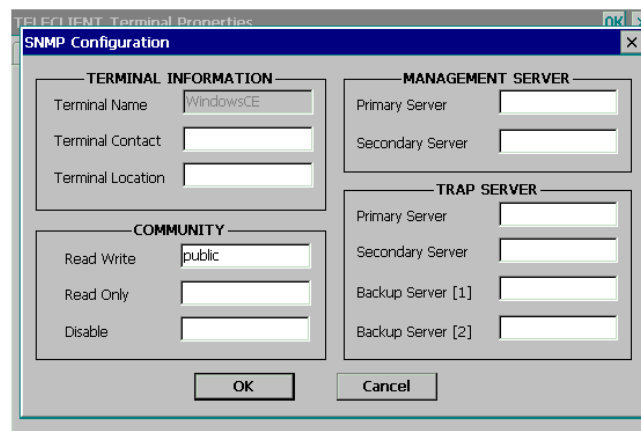
Figure 4.56 Management - SNMP
