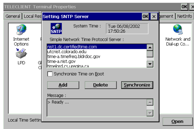
Figure 4.47 SNTP Settings
