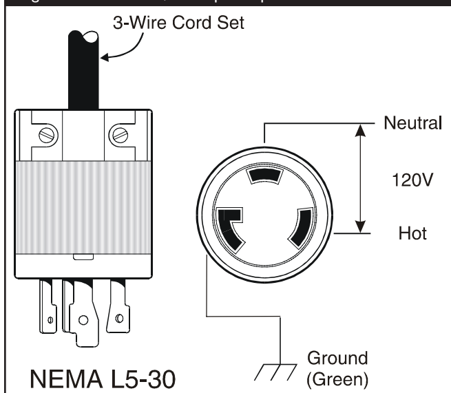
Figure 12 — 120 Volt, 30 Amp Receptacle
