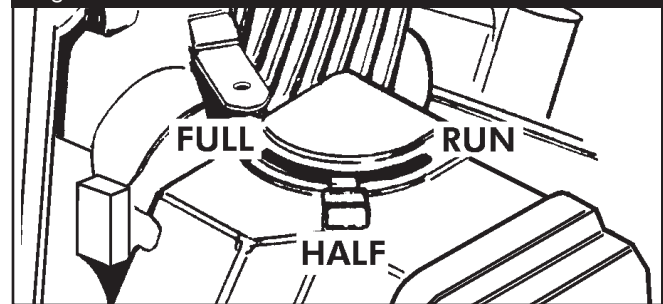
Figure 7 — Choke Positions
