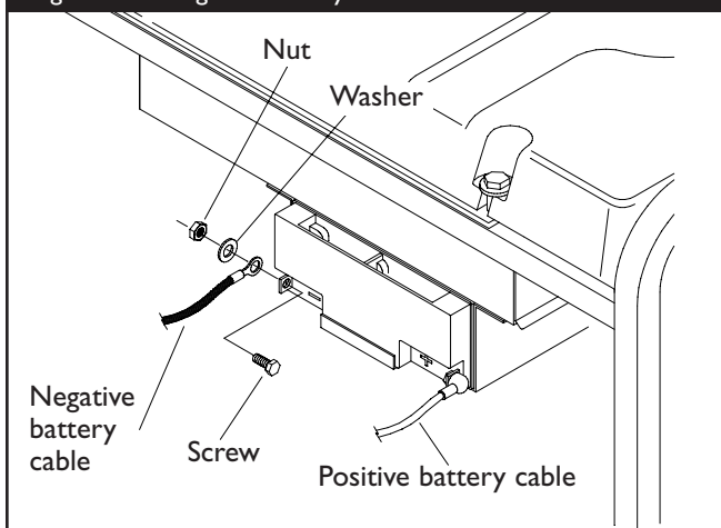
Figure 2 — Negative Battery Connection
