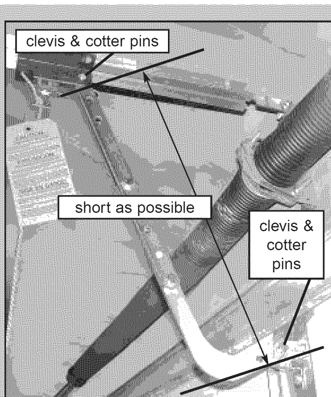
FIG. 2-10 Attaching door arms (sectional doors)
