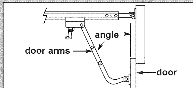
FIG. 2-11 Door arms at angle to door.
