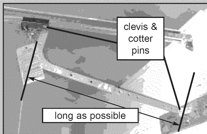
FIG. 2-12 Attaching door arms (1-piece doors)
