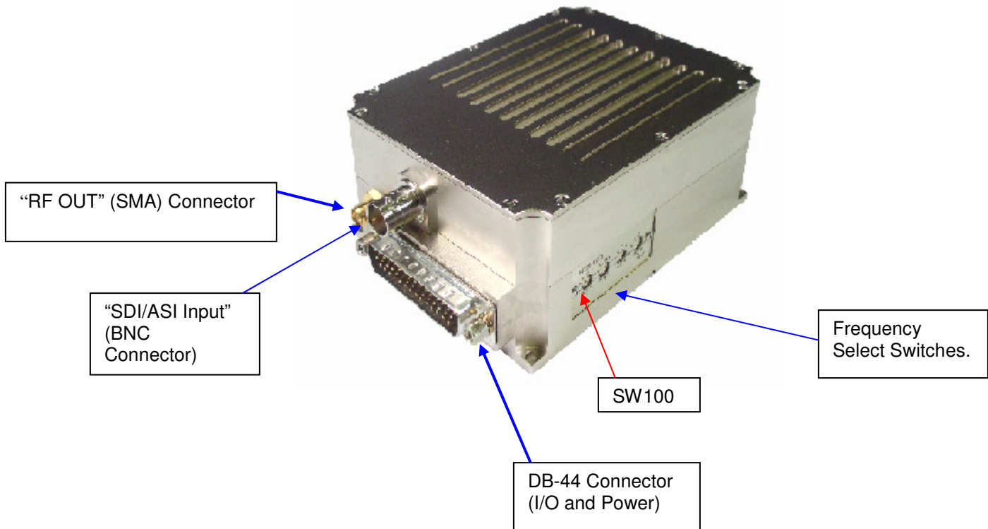
Figure 1 - MDT-B Connectors
