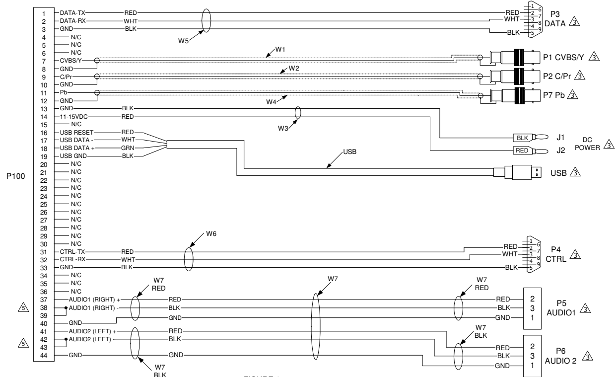
FIGURE 1 CABLE WIRING DIAGRAM
