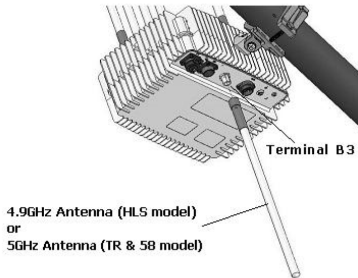
Figure 9: 5 GHz or 4.9GHz Third Band Antenna Installation
