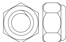
M10 Nylon Locknut (84)–4
