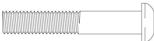
M10 x 60mm Button Screw (66)–2
