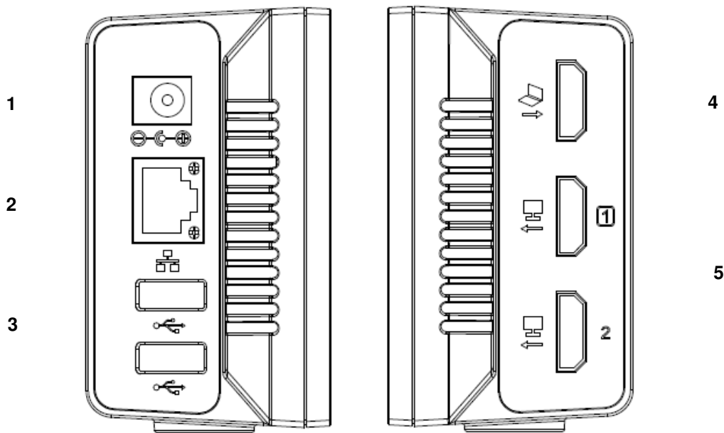
Figure 3: GVC3210Right/Left Panel
