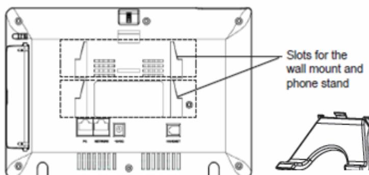
Figure 4: Phone Stand for GXV3174
