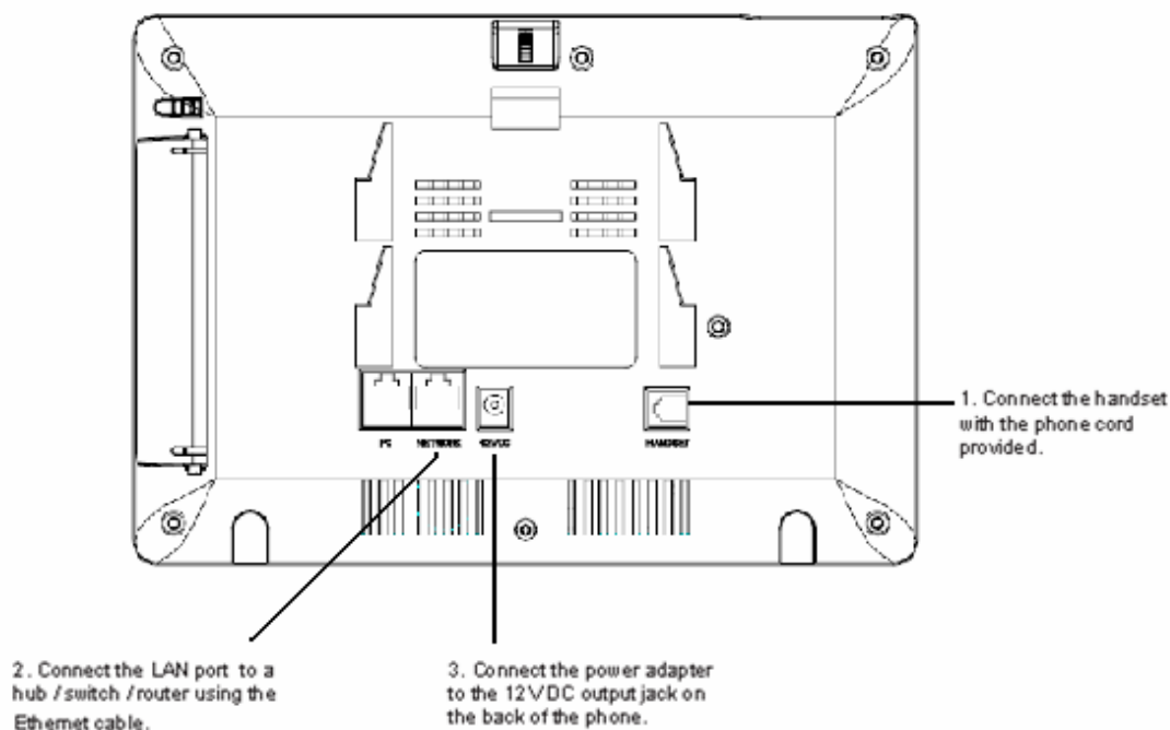
Figure 5: Connecting the GXV3174
