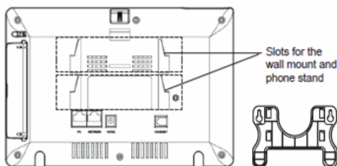
Figure 3: Wall Mount for GXV3174
