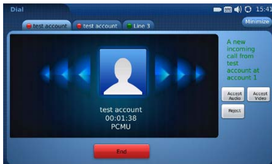
Figure 31: Multiple Calls
