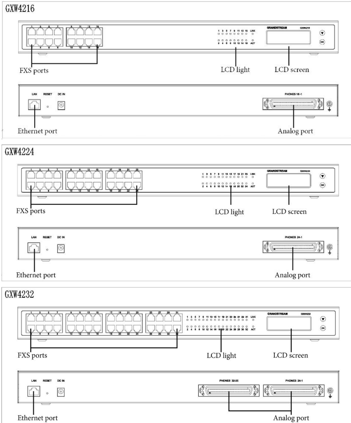
FIGURE 1: DIAGRAM OF GXW42XX FRONT & BACK PANEL
