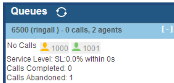
Figure 71: Queue Status
