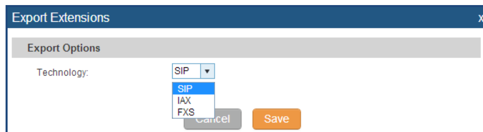
Figure 22: Export Extensions
