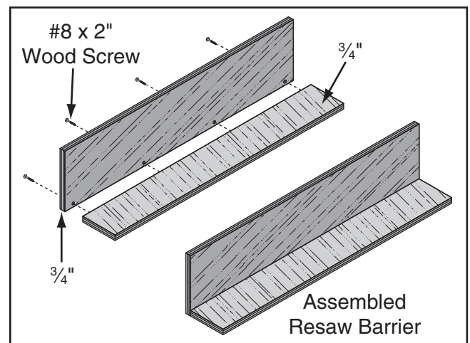
Figure 59. Resaw barrier.
