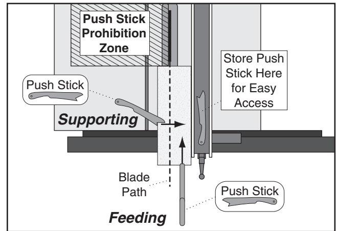
Figure 69. Using push sticks to rip narrow stock.
