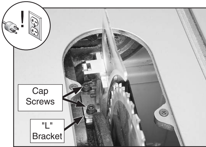
Figure 112. Cap screws for adjusting spreader/ripping knife position.
