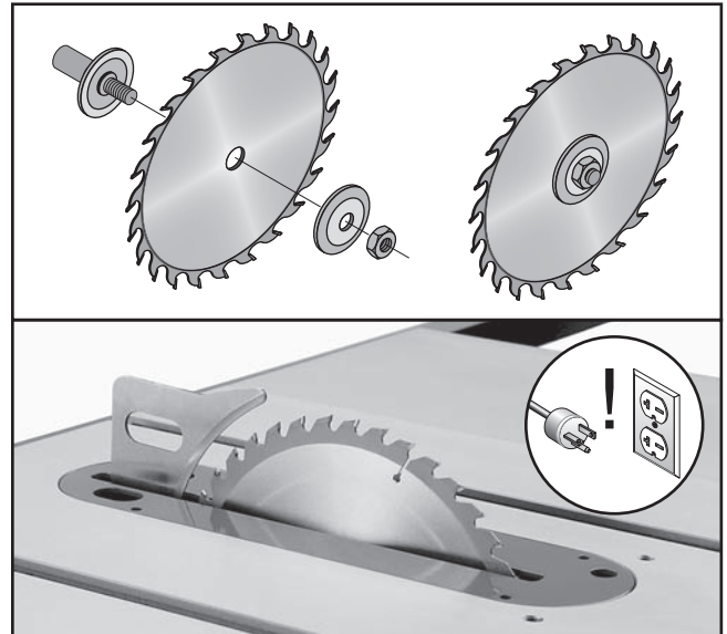
Figure 37. Blade order of installation and teeth facing the correct direction.
