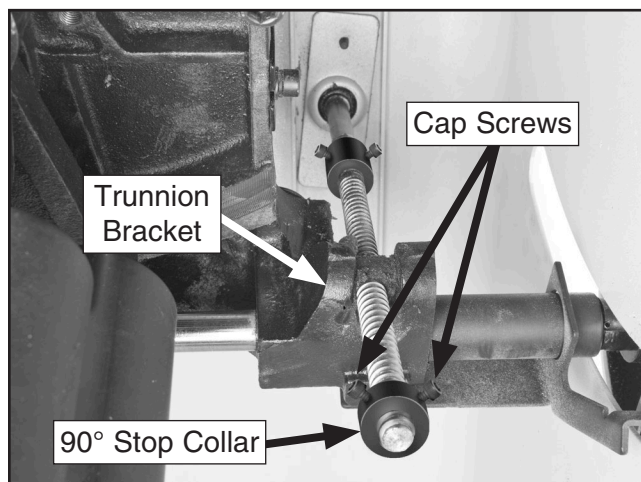
Figure 100. 90° stop bolt and jam nut.
