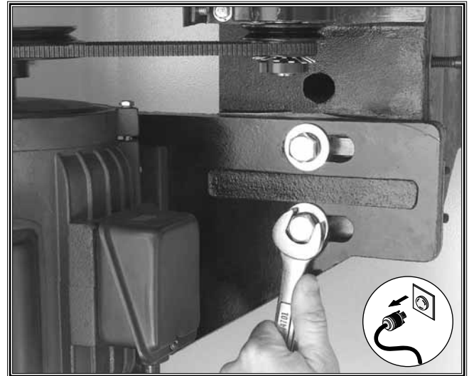
Figure 30. Loosening spindle slide bolts.
