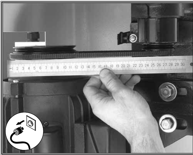
Figure 26. Use straightedge to check V-belts.
