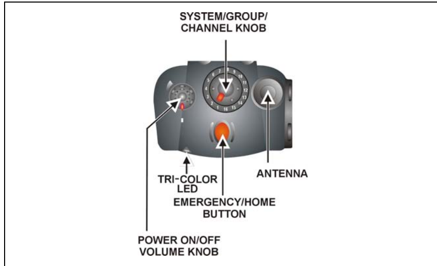
Figure 3: Top View
