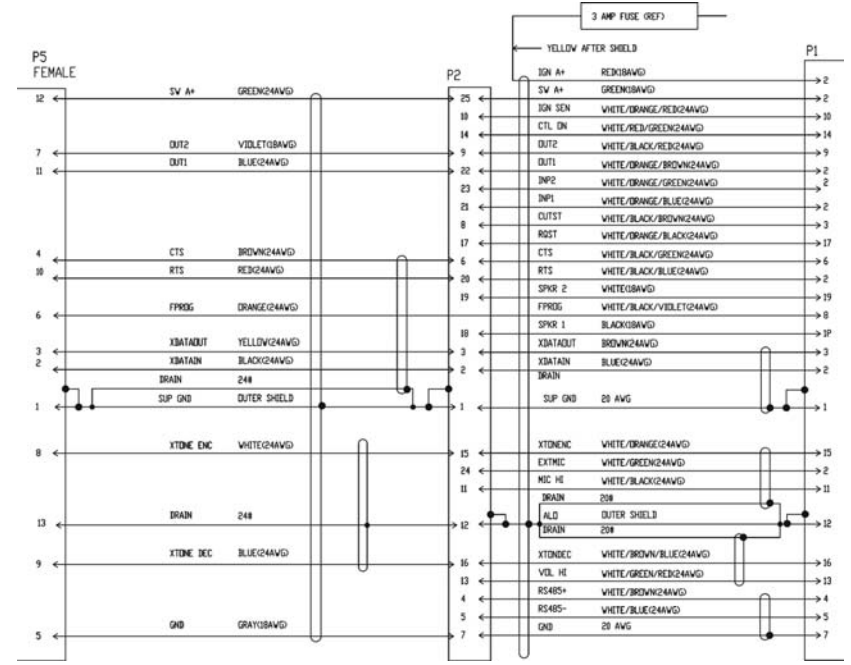
Figure 9-6: Remote Extended Option Control Cable (CA101288V4)
