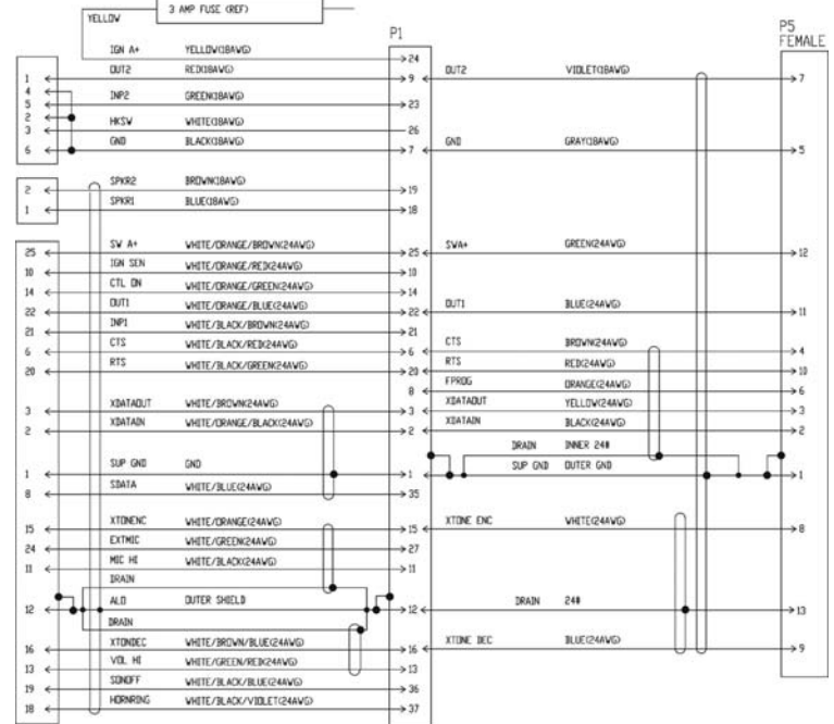
Figure 9-4 - Front Mount Extended Option Accessory Cable CA101288V2
