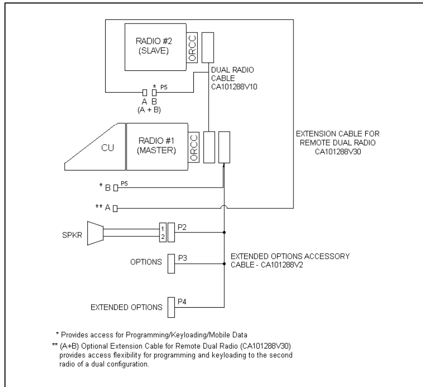
Figure 31 - M7100 HP Dual Radio Front Mount/Remote Mount Installation Configuration
