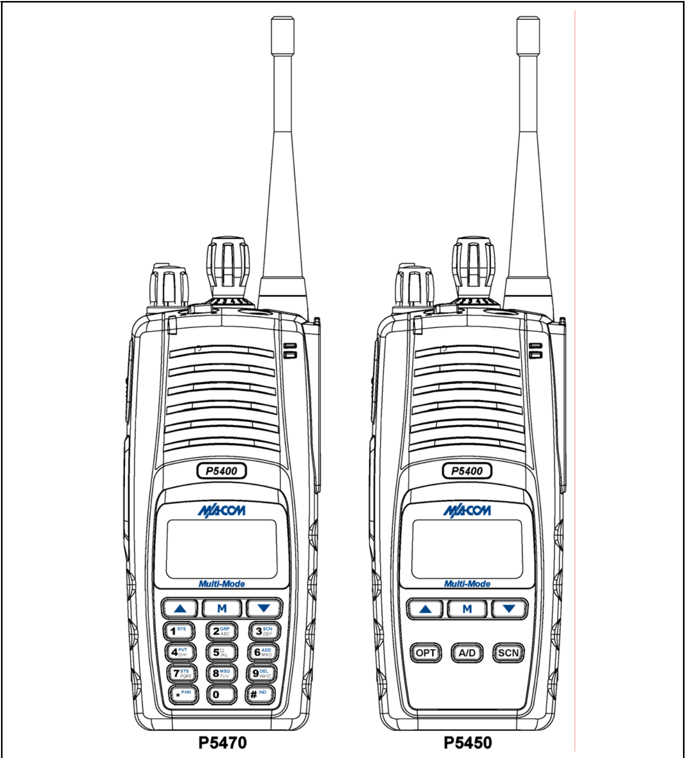
Figure 7-1: P5400 Portable Radio
