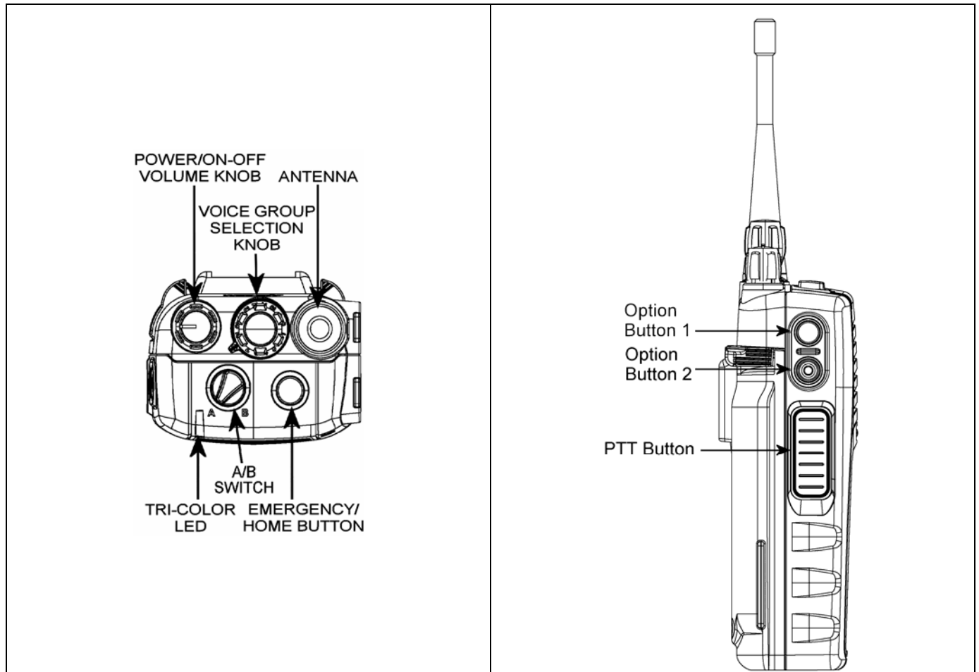
Figure 9-1: Top View
