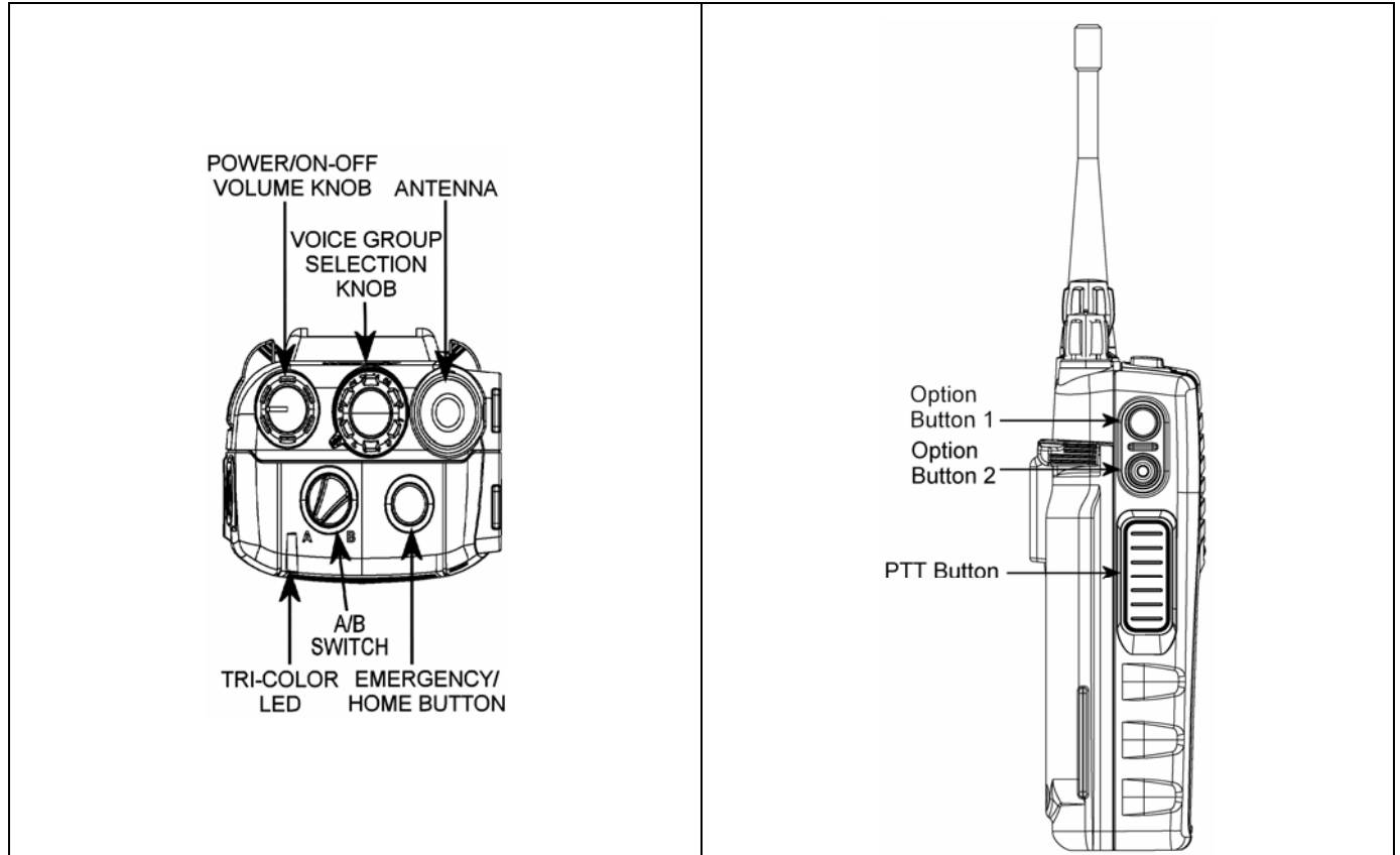
Figure 10-1: Top View
