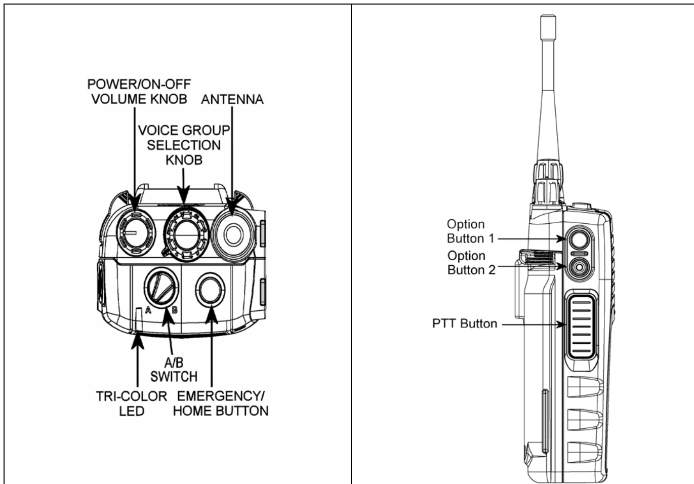
Figure 9-1: Top View
