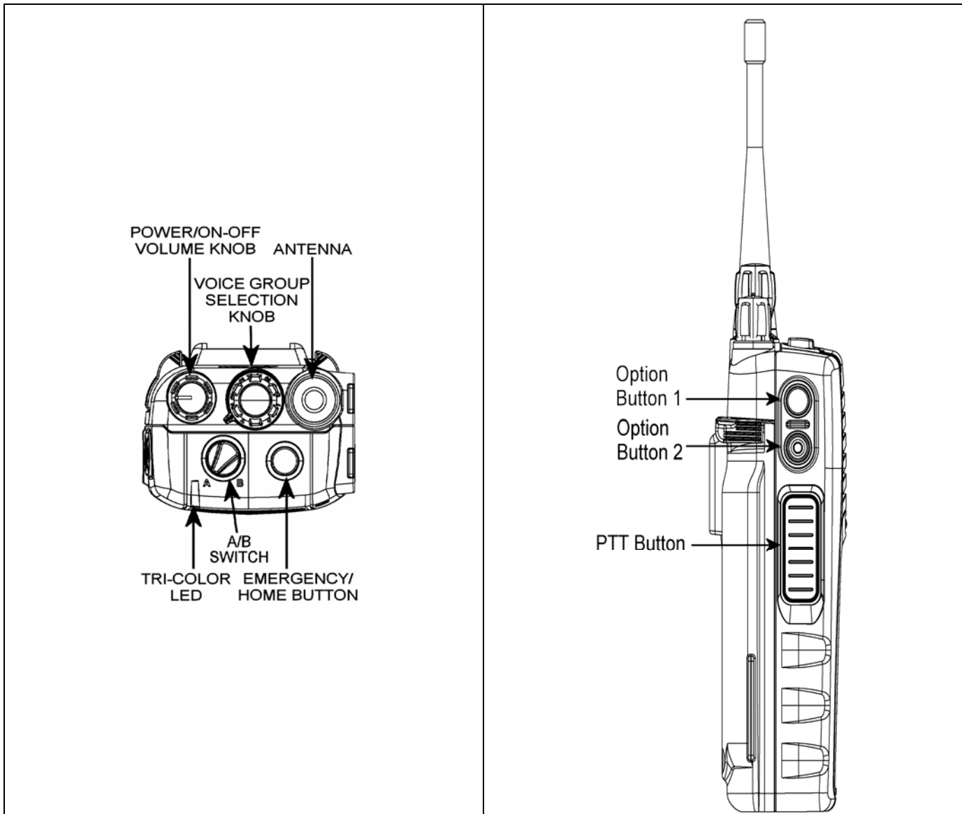
Figure 9-1: Top View
