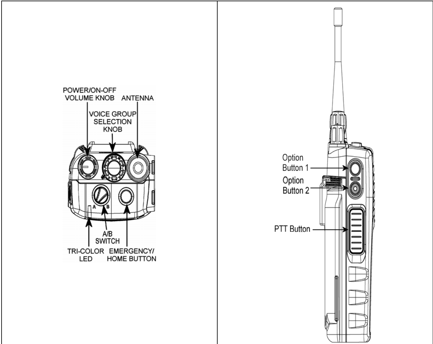
Figure 10-1: Top View
