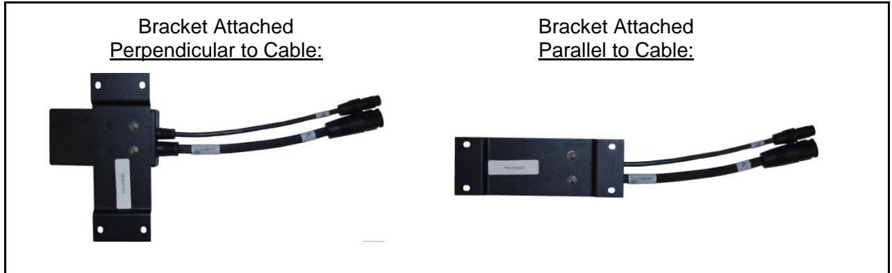
Figure 9-14: HHC-731 Interface Cable Mounting Bracket-to-Cable Positioning
