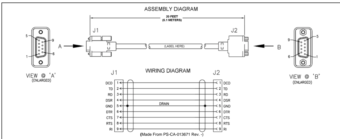
Figure 12-5: Serial Data Cable CA-013671-020
