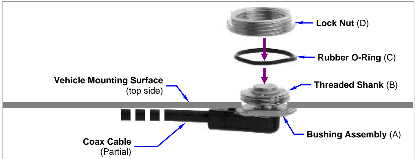
Figure 7-5: Installing a Standard 3/4-Inch NMO Antenna Mount (e.g., AN-125001-001 or AN-125001-002)
