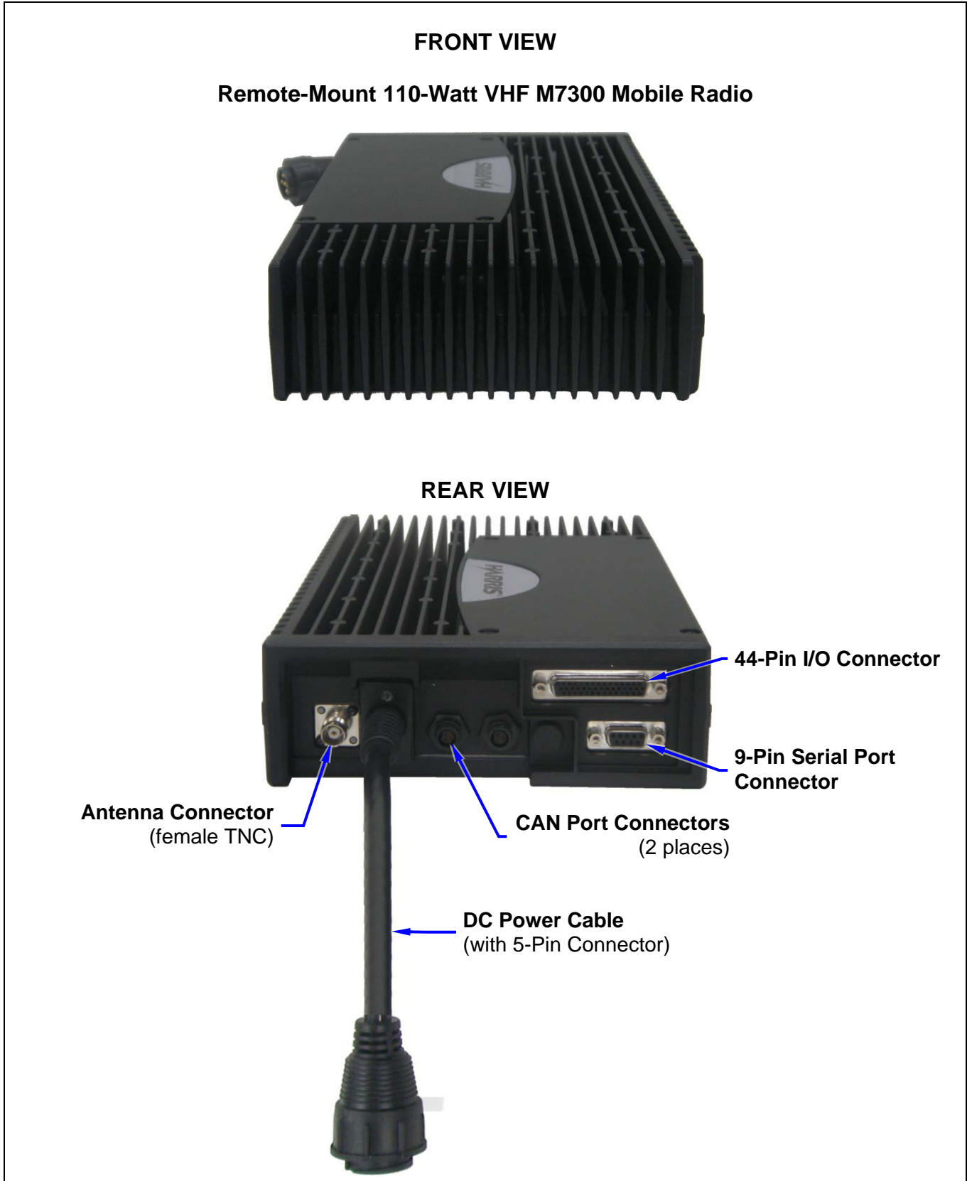
Figure 6-2: M7300 Remote-Mount 110-Watt Mobile Radios — Front and Rear Views
