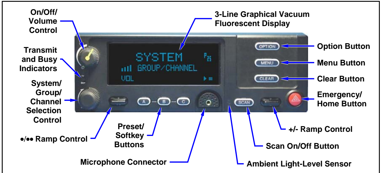
Figure 9-5: CH-721 Scan Model Control Head Front Panel
