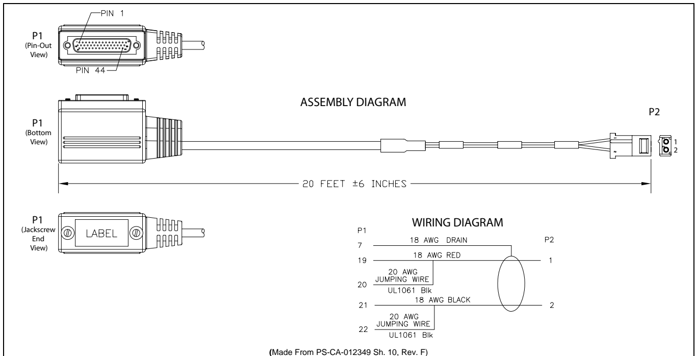
Figure 12-8: Speaker-Only Option Cable CA-012349-007
