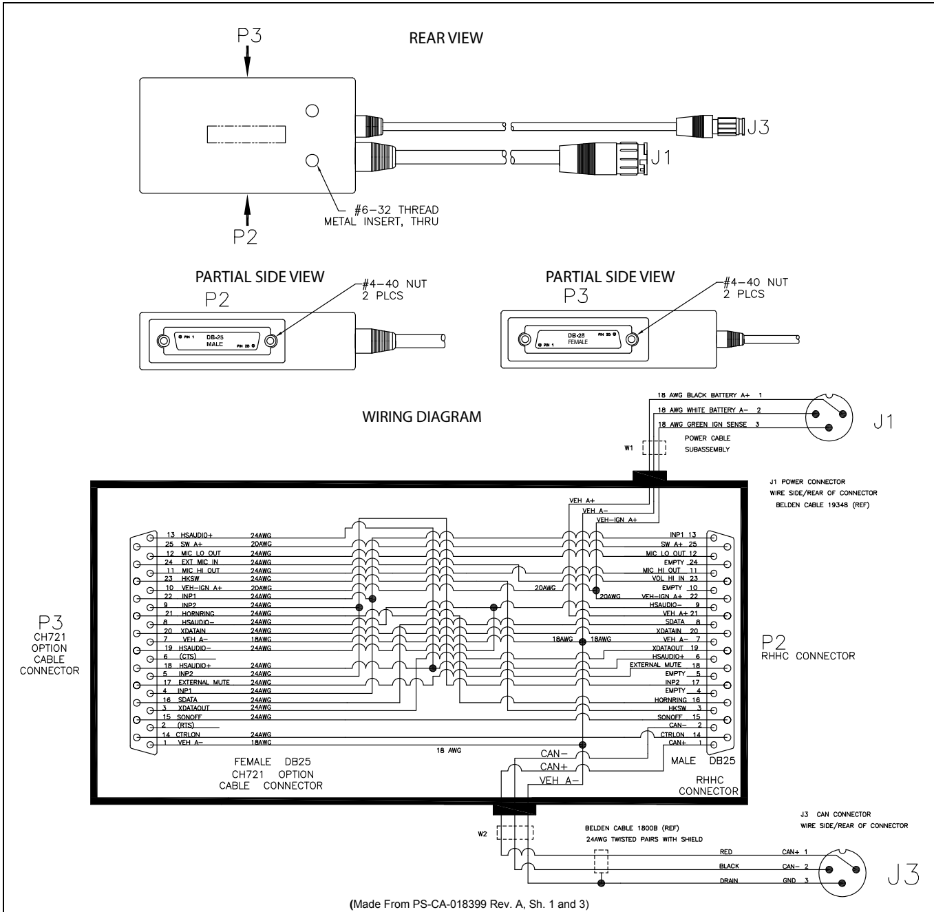
Figure 11-5: HHC-731 Interface Cable CA-018399-001
