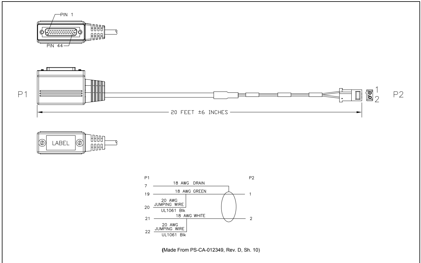
Figure 11-6: Speaker-Only Option Cable CA-012349-007
