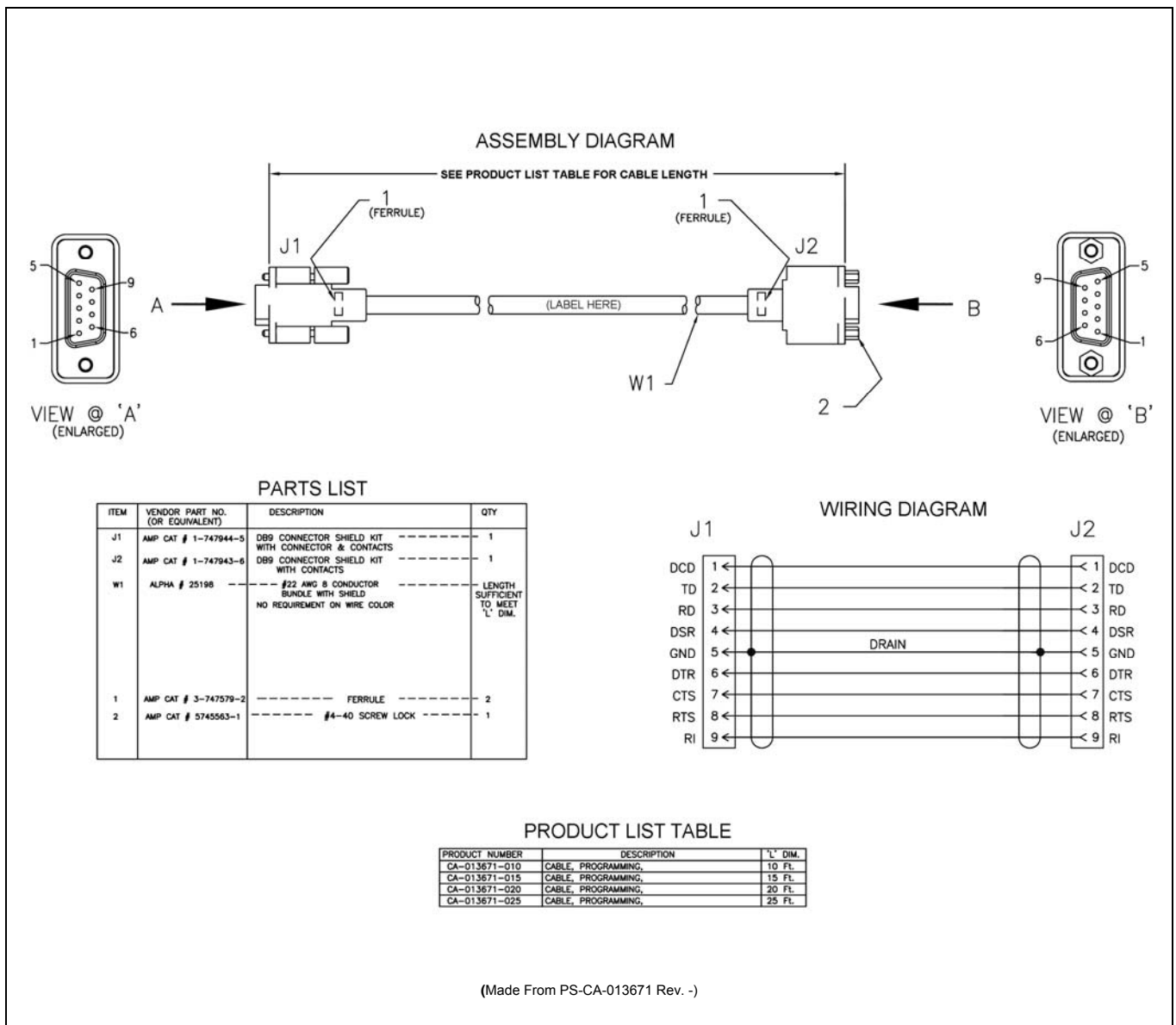
Figure 11-2: Serial Programming Cable CA-013671-020
