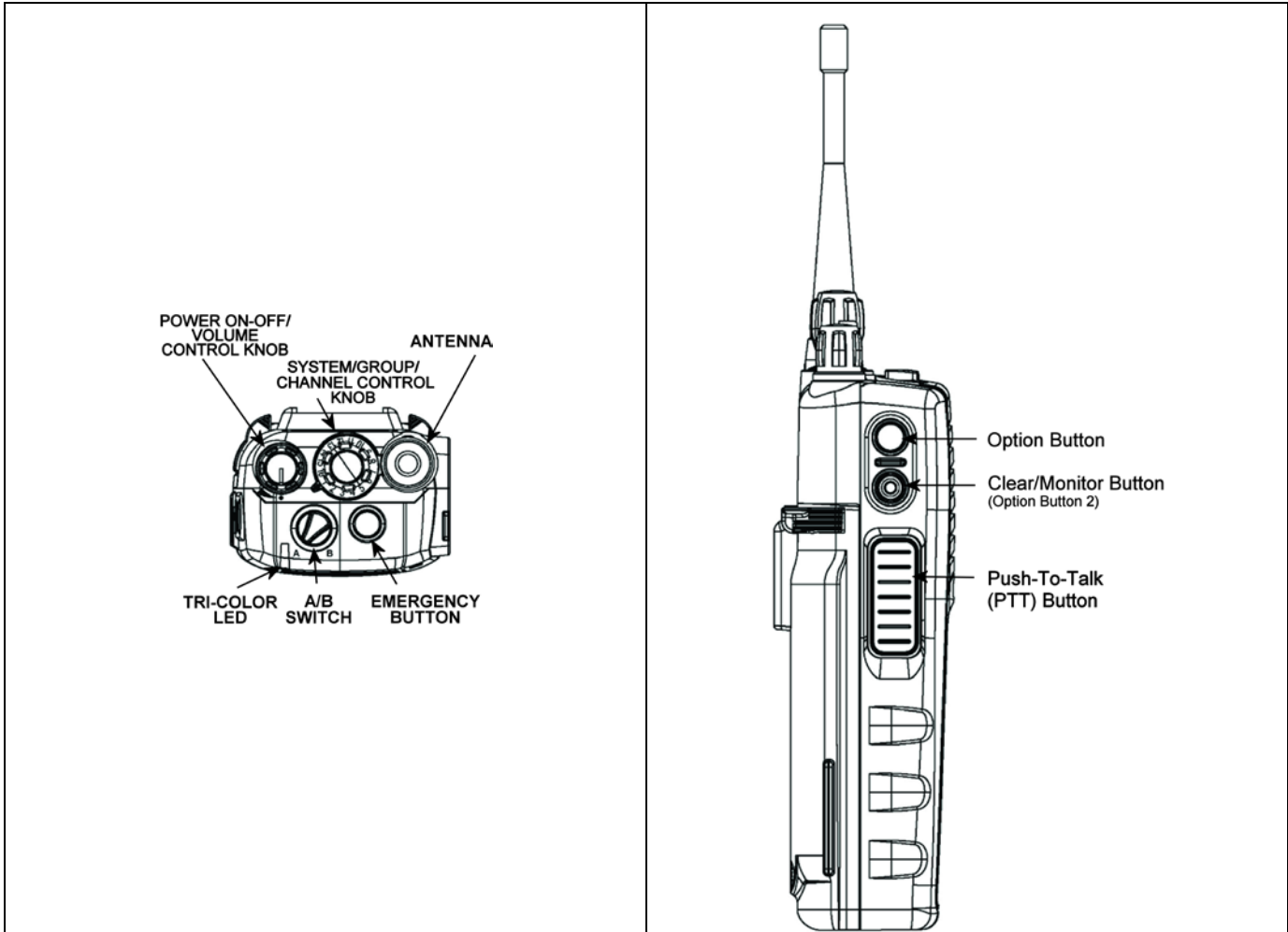
Figure 7-1: Top View
