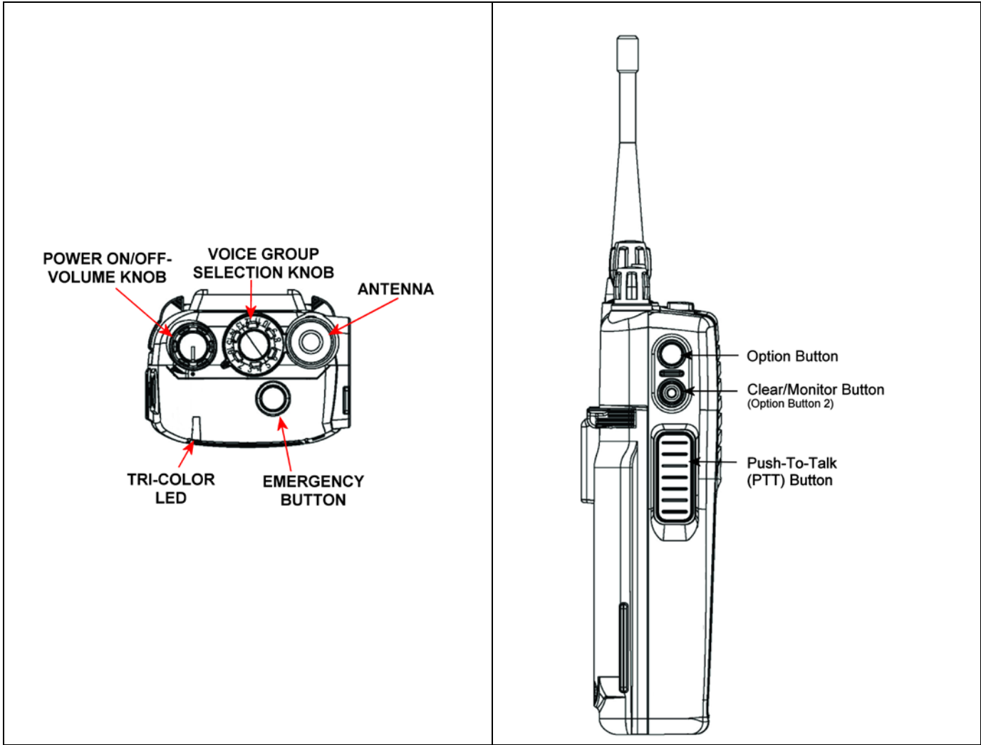
Figure 7-1: Top View
