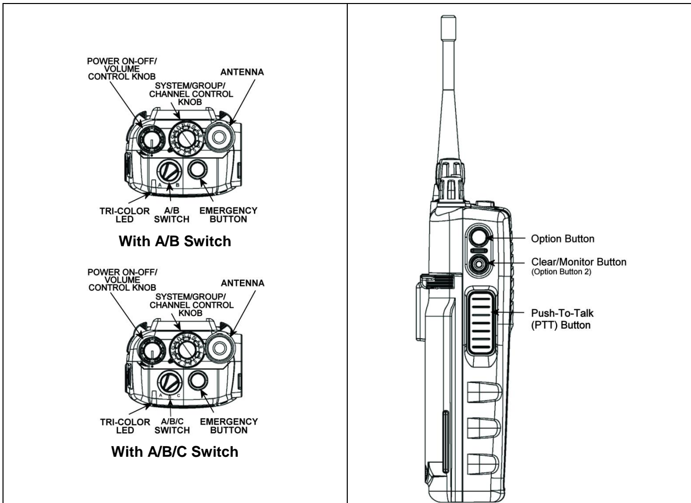
Figure 8-1: Top View
