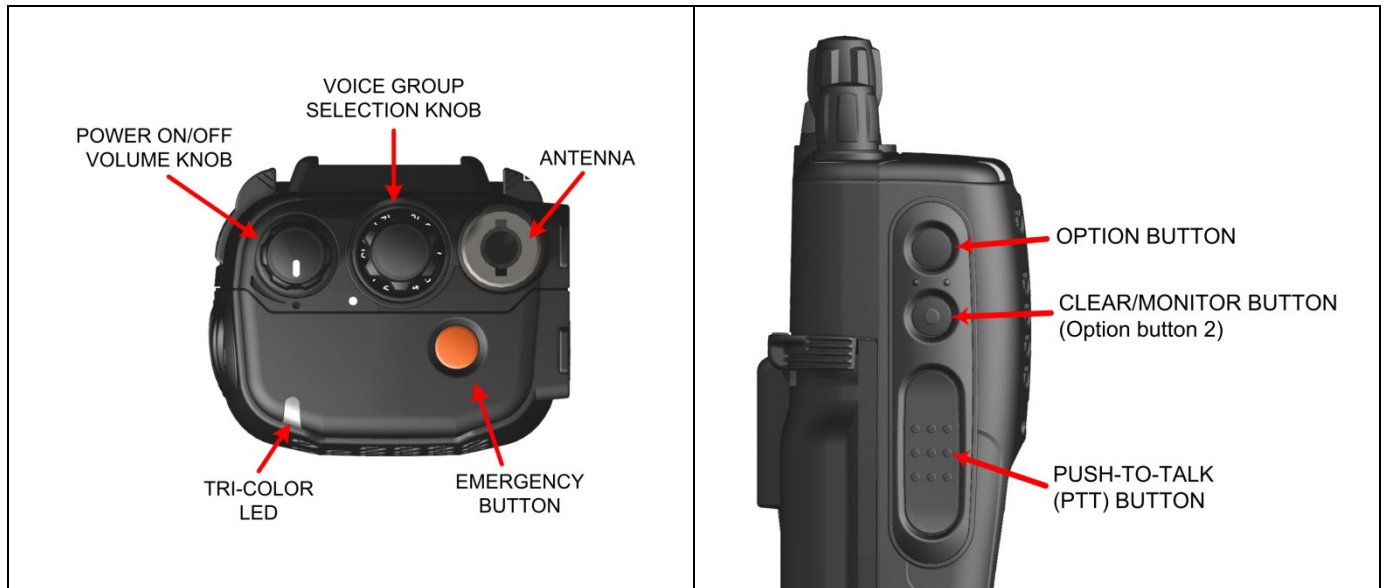
Figure 8-1: Top View
