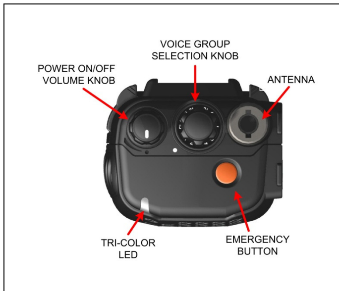
Figure 7-1: Top View
