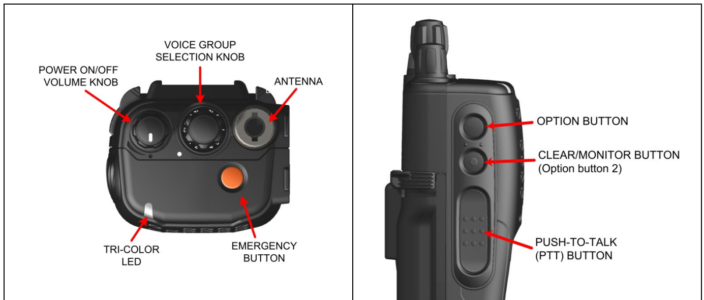
Figure 8-1: Top View
