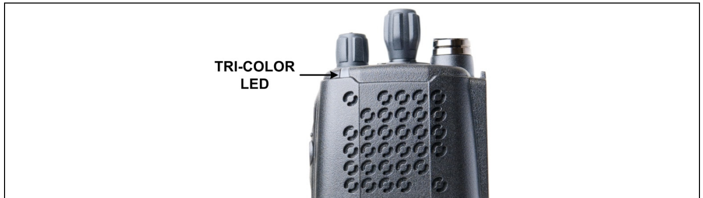
Figure 8-7: Tri-Color LED
