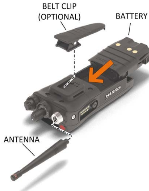
Figure 4-1: Radio Assembly
