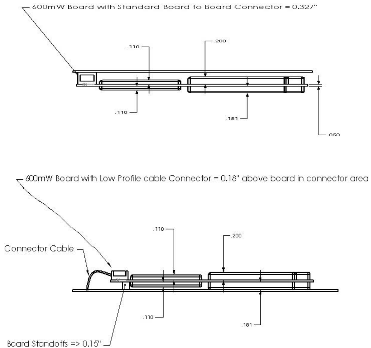
Figure 1.4-1 Module Mounting Configuration
