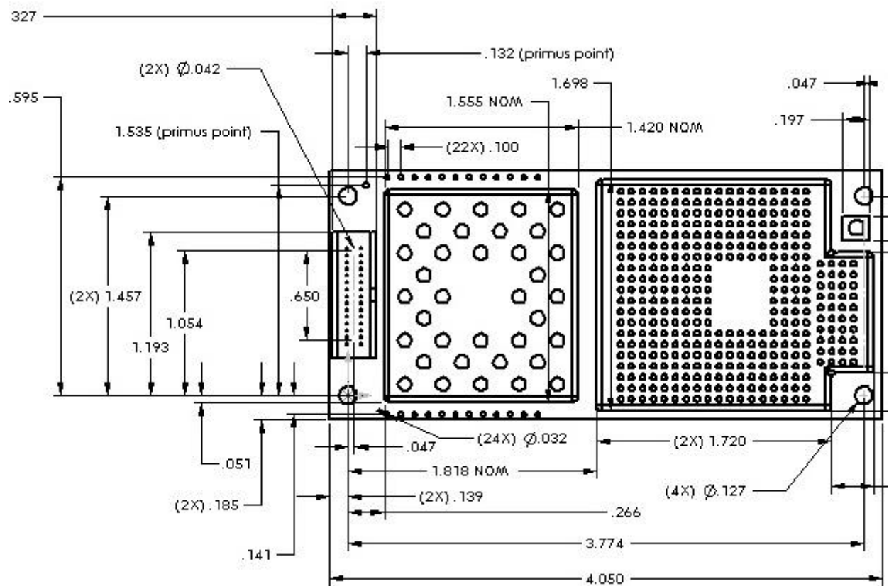
Figure 2.1-1 Module Dimensions
