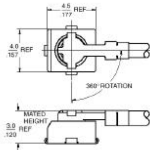
Pigtail Assembly
