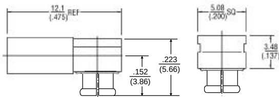
Right Angle Crimp Jack
