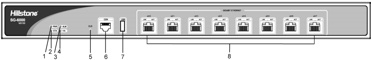
Figure 1-11: SG-6000-M3100 Front Panel
