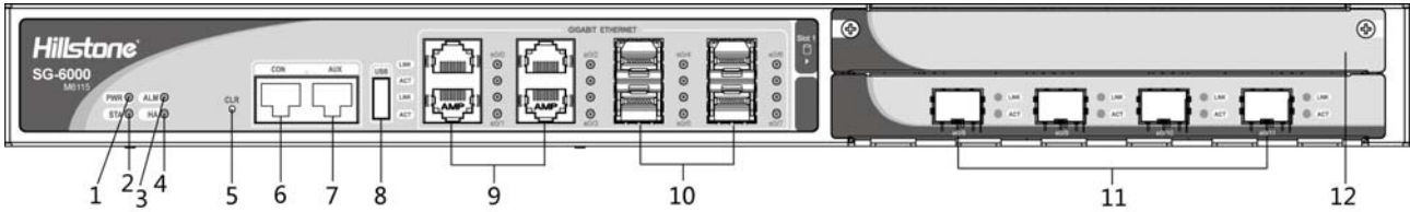
Figure 1-7: SG-6000-M6115 (single power supply) Front Panel
