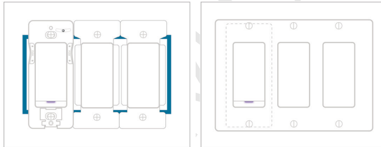
FIGURE 5: DIRECT GANG BOX INSTALLATION
