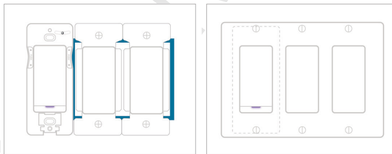
FIGURE 3: ADJACENT GANG BOX INSTALLATION
