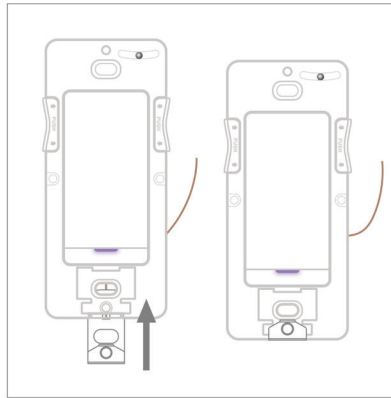
FIGURE 4: GROUND WIRE INSTALLATION
