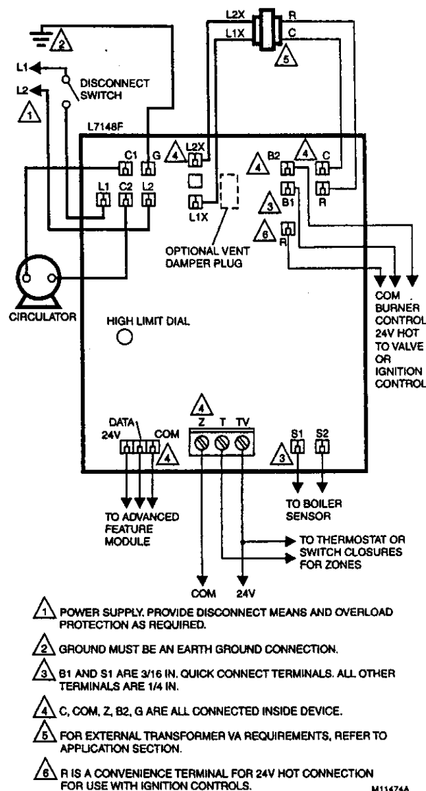
Fig. 2. External connections for L7148F.
