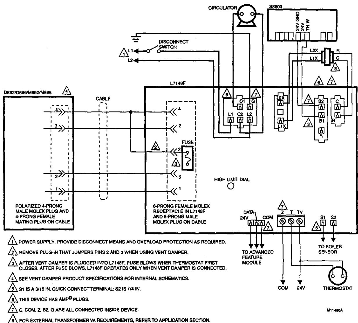
Fig. 7. Wiring L7148F with AMP® plug connections and internal plug directly to D892/D896/M892/M896 Vent Damper in hydronic intermittent pilot system.
