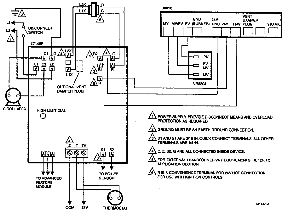
Fig. 6. Wiring L7148F with S8610 Intermittent Pilot Ignition Module with automatic vent damper plug and Honeywell D892/D896/M892/M896 Vent Damper.
