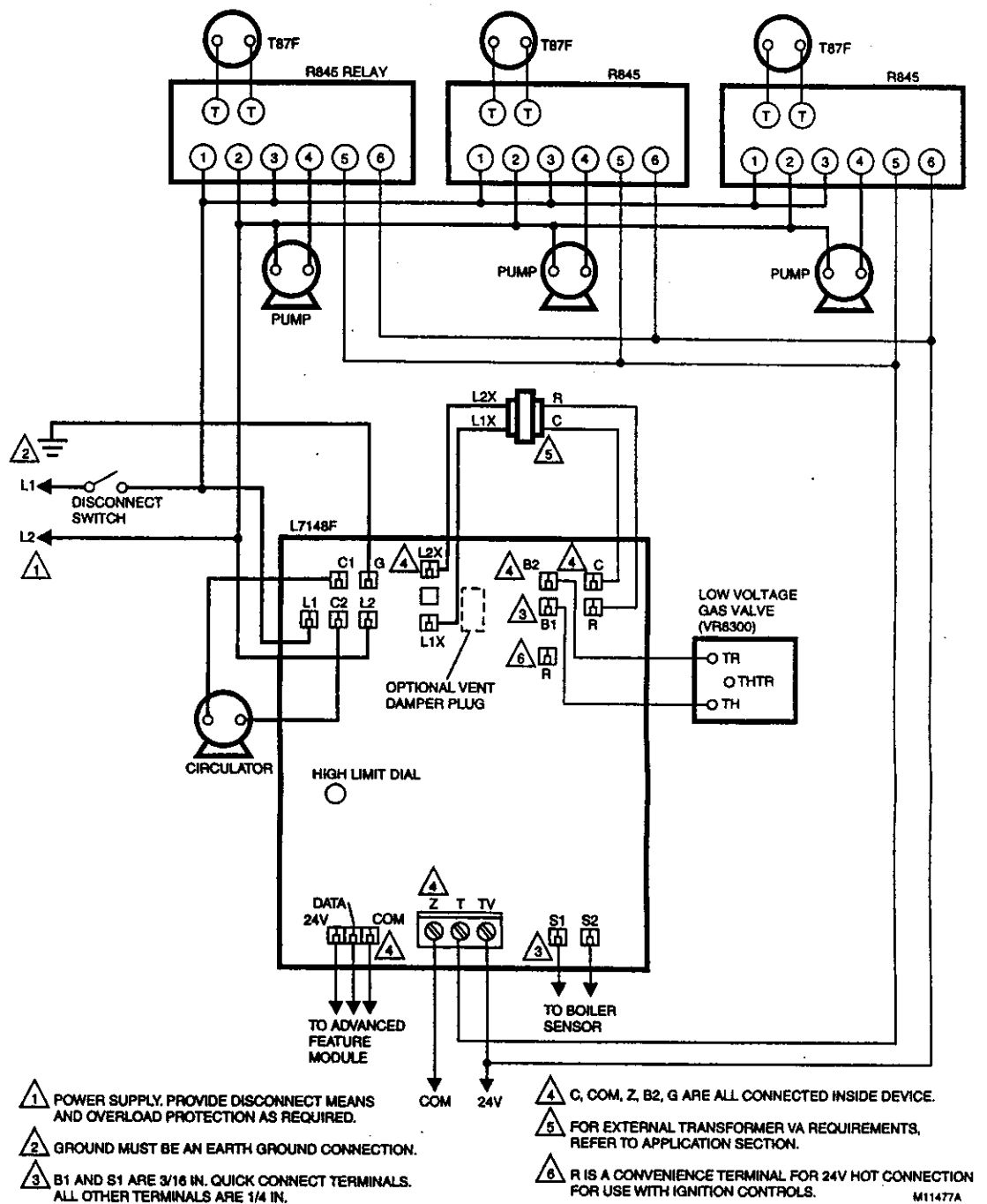
Fig. 4. Wiring L7148F in a gas-fired, forced hot water, zoned, pump system.
