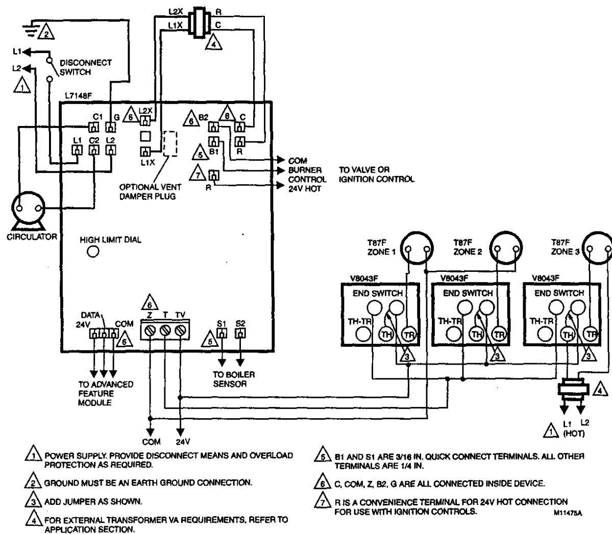
Fig. 3. Wiring L7148F with multizone valves.
