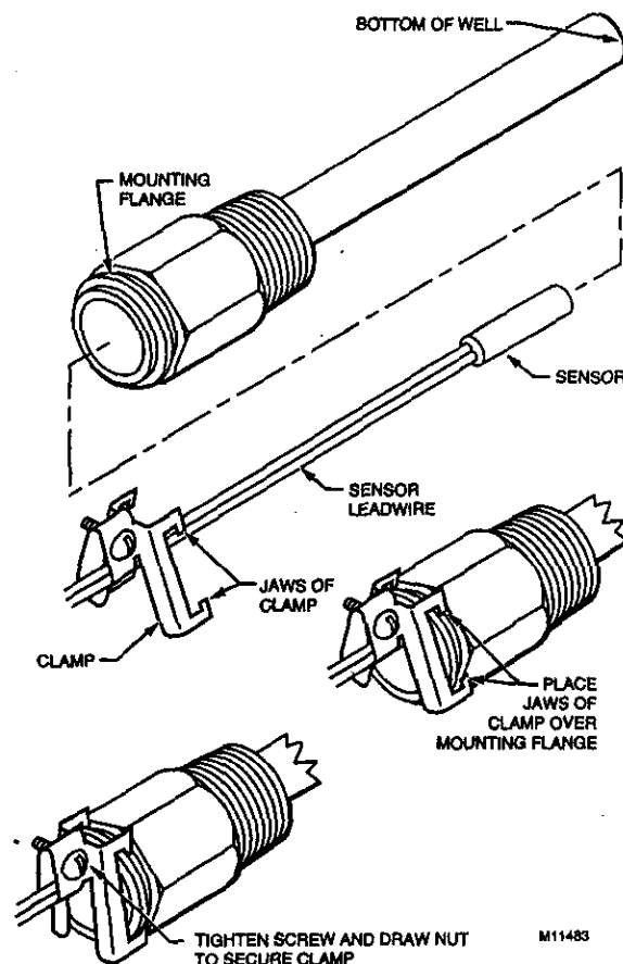
Fig. 1. Secure sensor and leadwire with mounting clamp.
