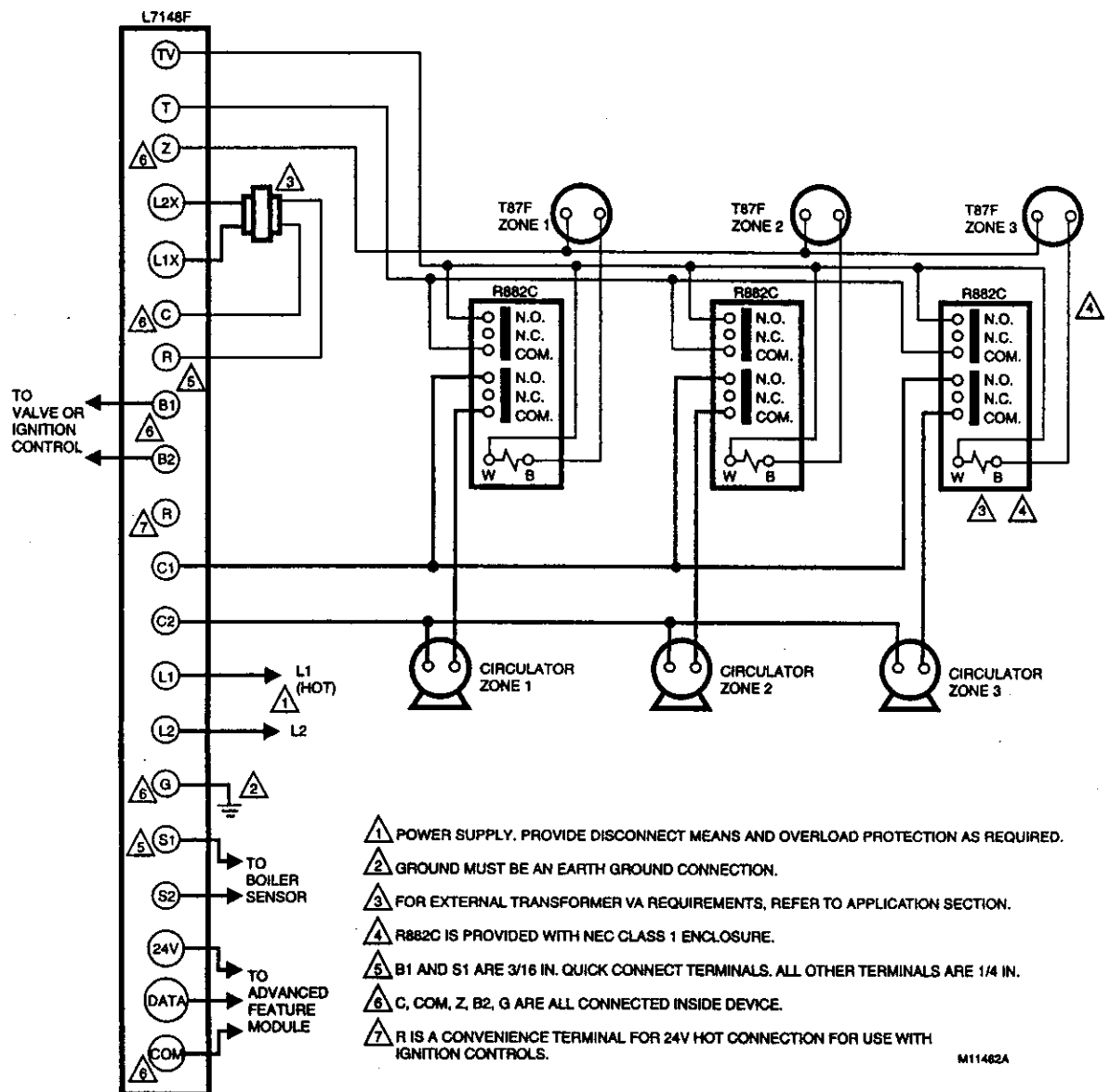
Fig. 8. Multizone system with R882C switched circulator.
