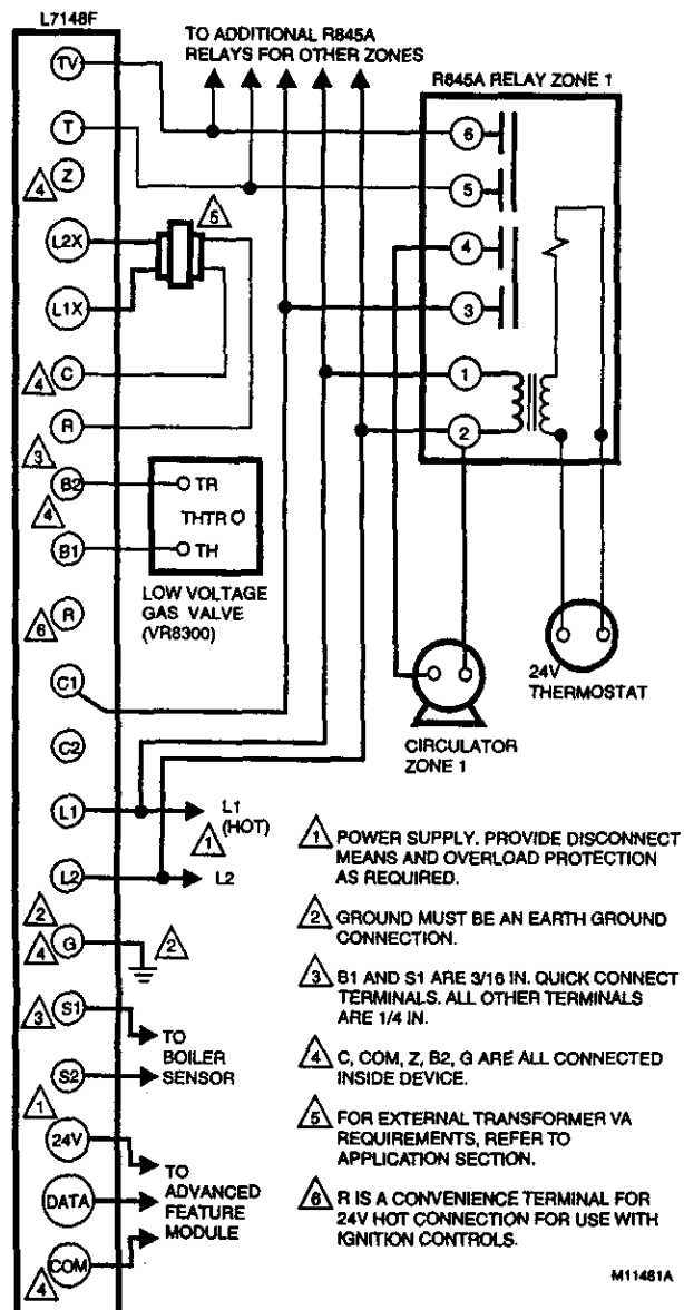
Fig. 5. Wiring L7148F in multizone system with R845 switched circulator.
