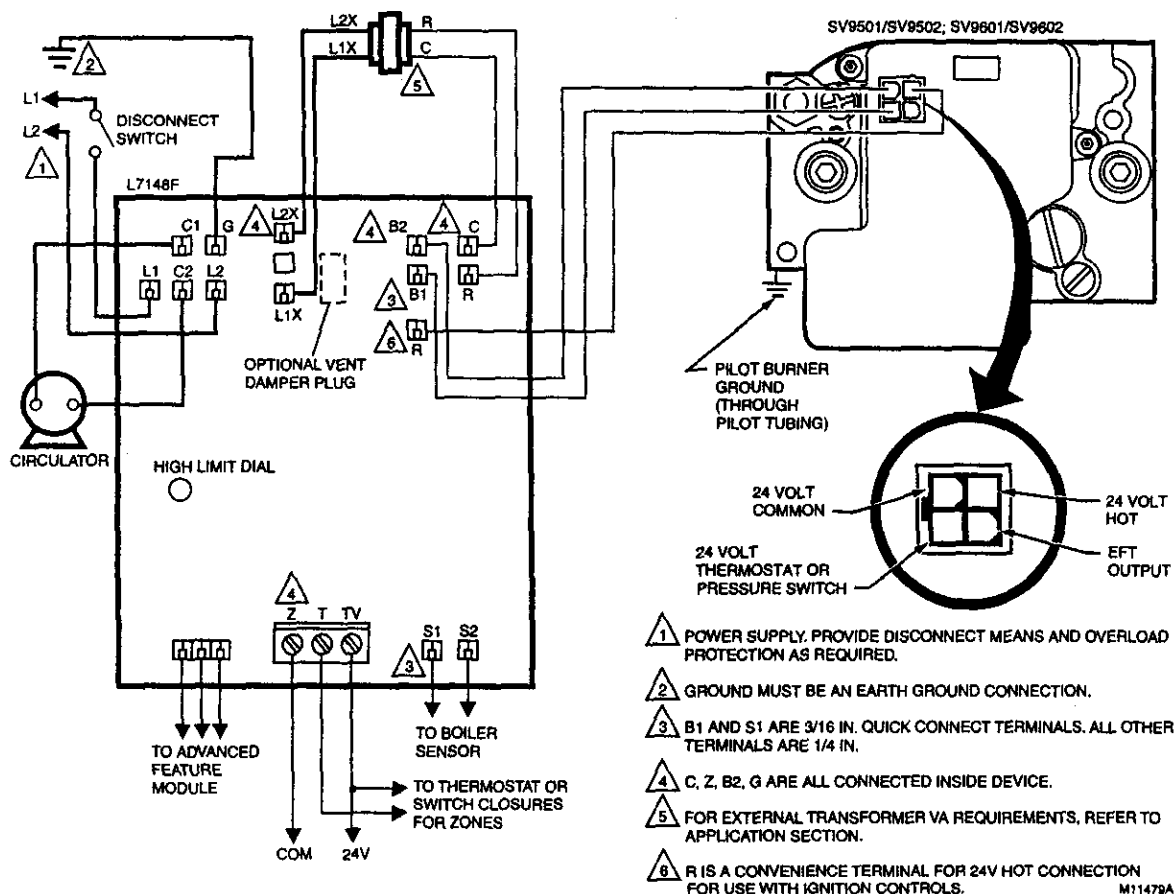
Fig. 9. Wiring L7148F with SV9501/SV9502/SV9601/SV9602 SmartValve™ System Controls.
