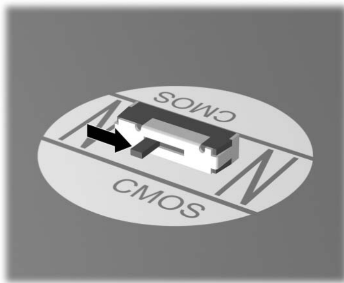
Interruptor CMOS
