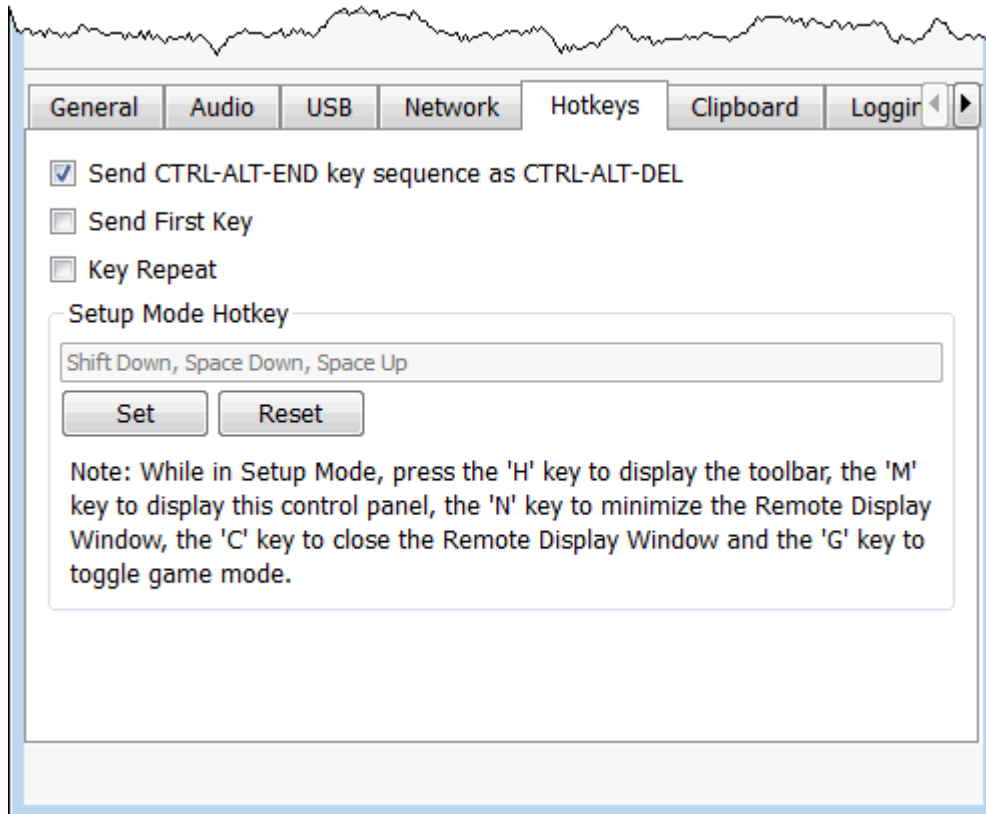
Figure 6-25 The Hotkeys tab options
