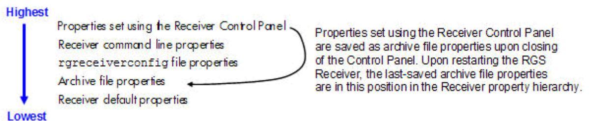
Figure 8-1 Receiver property hierarchy
