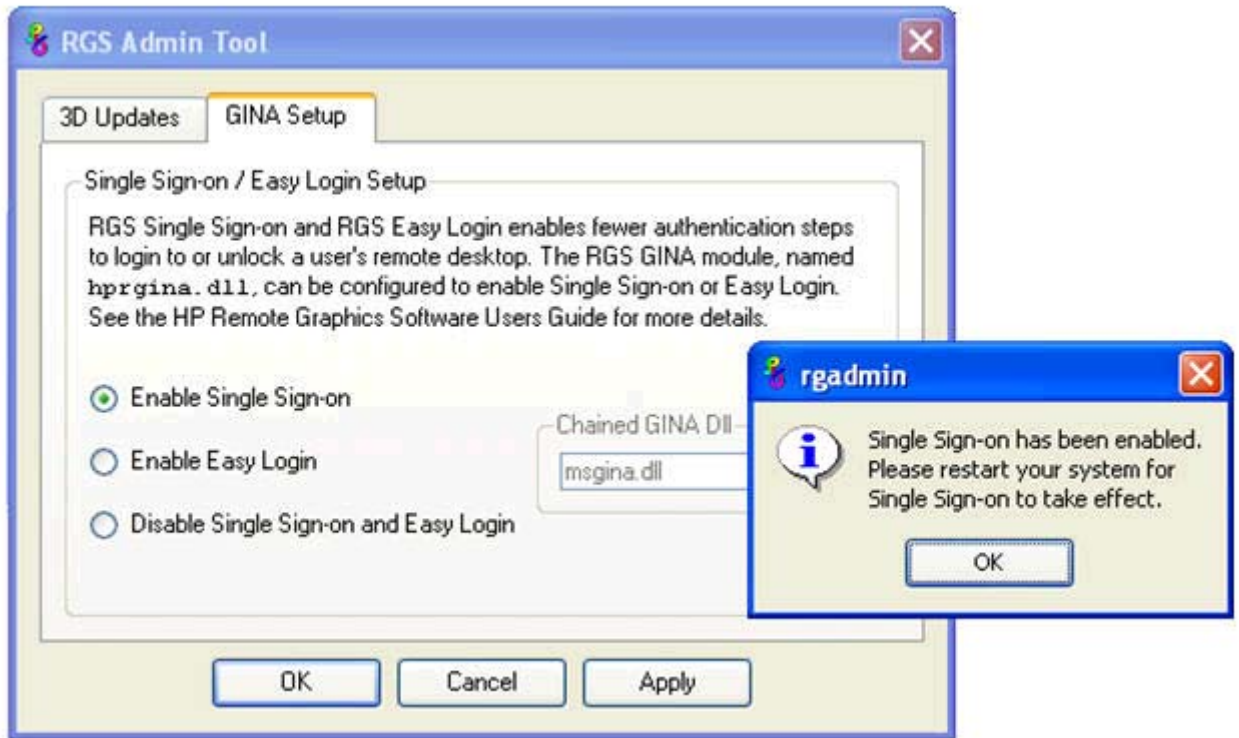
Figure 3-10 Using the rgsadmin tool to enable Single Sign-on (Windows Vista and Windows 7)
