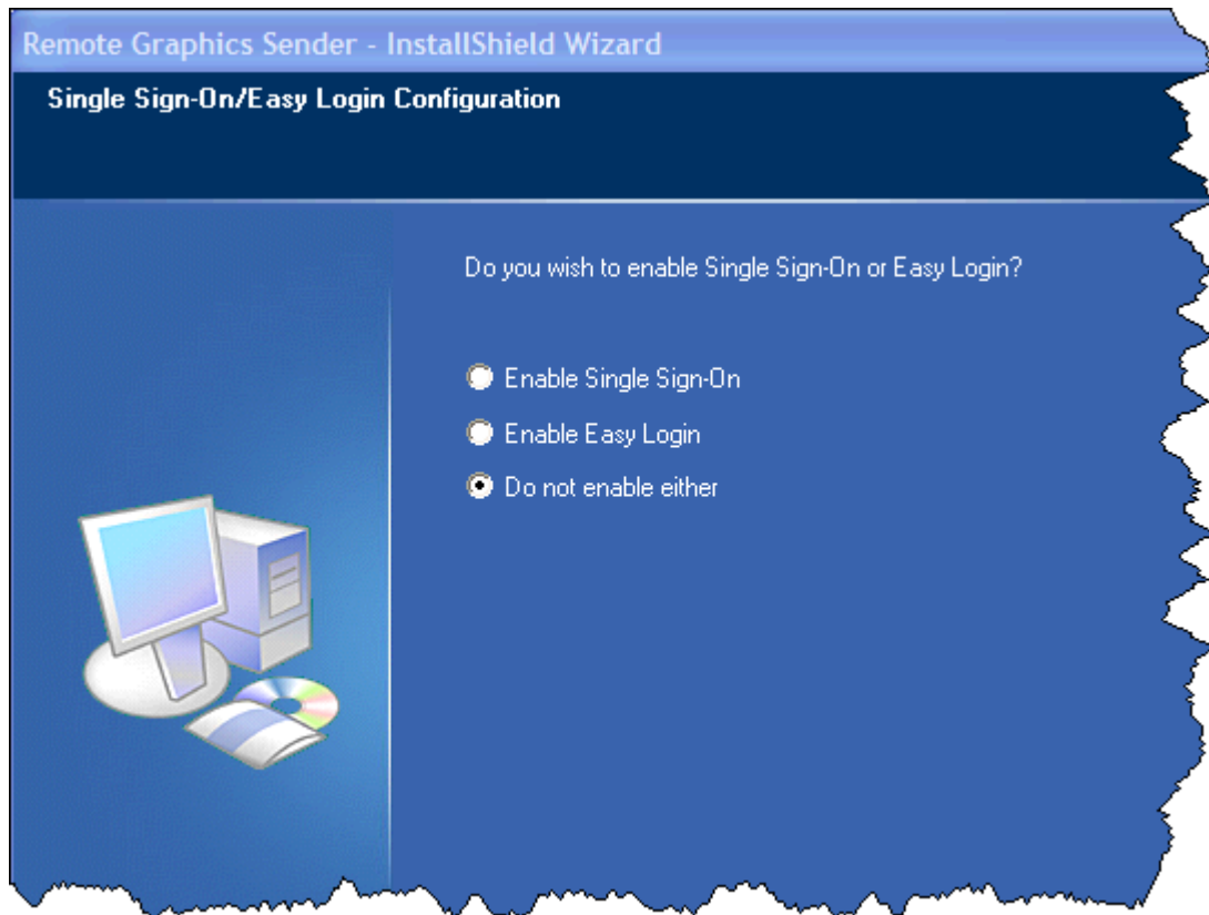
Figure 3-8 The dialog presented during Sender installation to enable Single Sign-on or Easy Login
