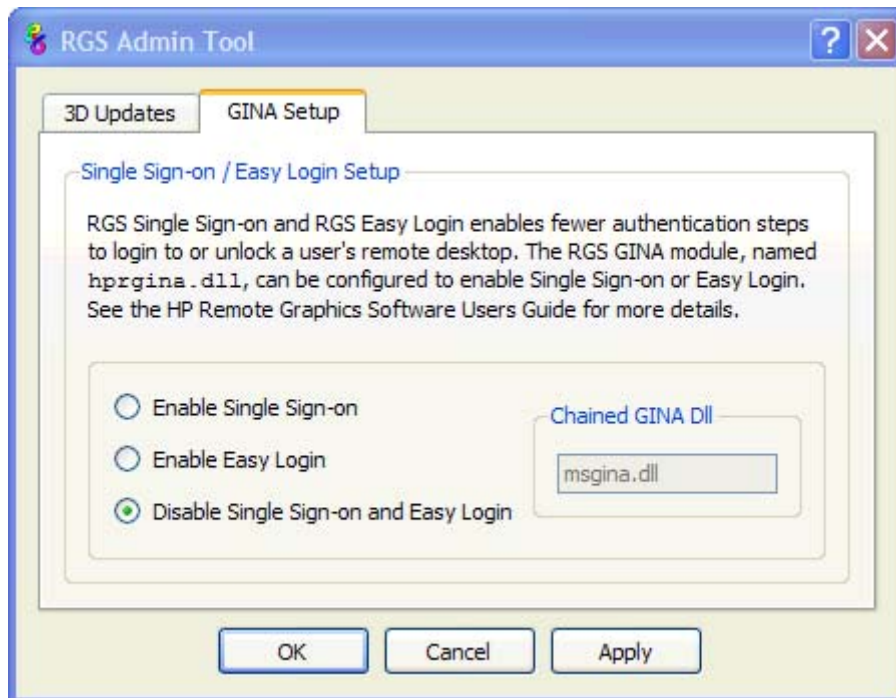
Figure 3-13 Using rgadmin to disable Single Sign-on (Windows XP Professional)
