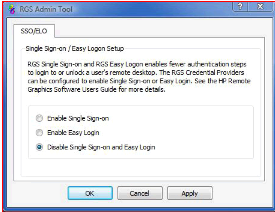
Figure 3-14 Using rgadmin to disable Single Sign-on (Windows Vista and Windows 7)
