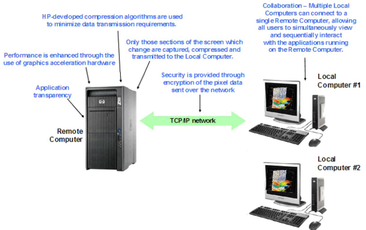
Figure 1-3 Features of HP RGS
