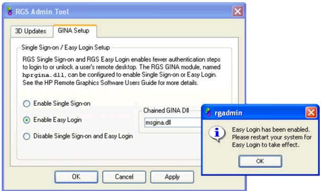
Figure 3-22 Dialog to enable or disable Single Sign-on and Easy Login (Windows XP Professional)
