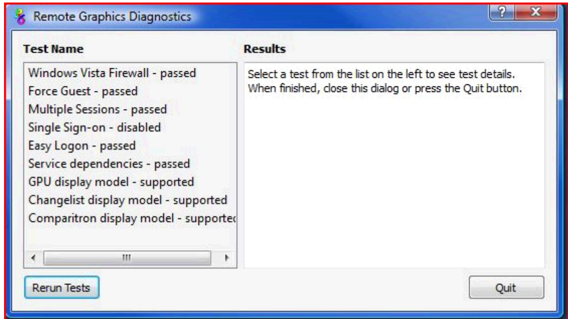
Figure 3-20 Output of the RGS Diagnostics Tool
