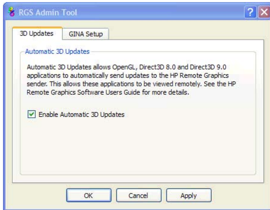
Figure 3-21 3D Updates tab
