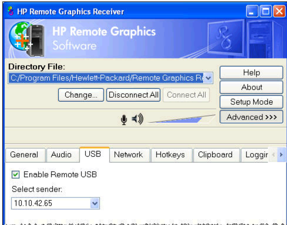
Figure 6-15 USB tab options
