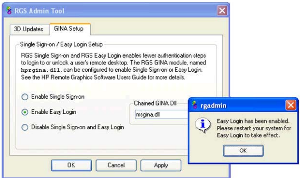
Figure 3-16 Using the rgadmin tool to enable Easy Login (Windows Vista and Windows 7)
