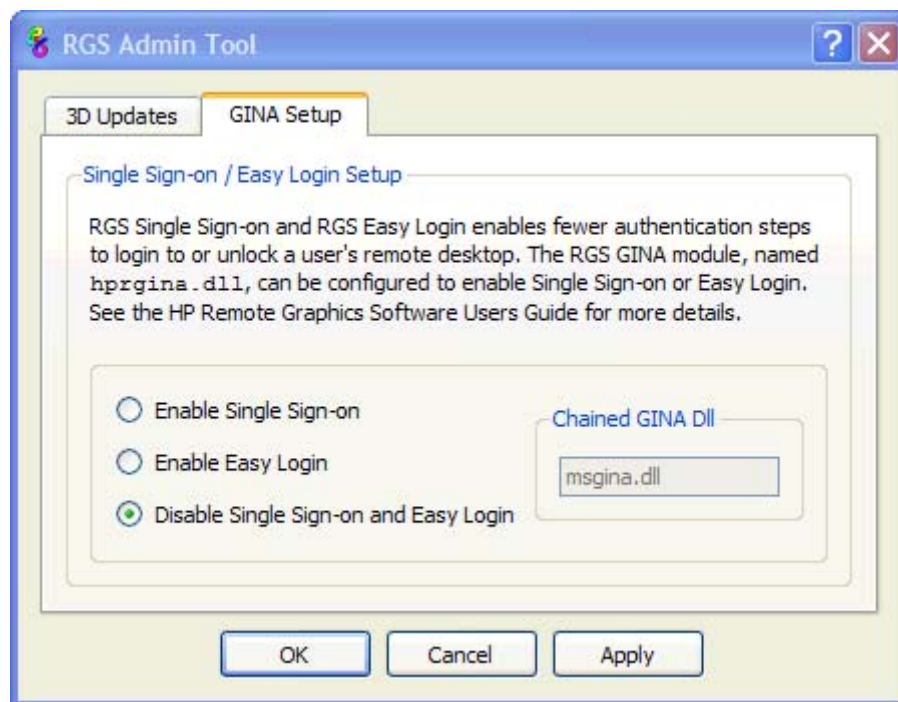
Figure 3-18 Using rgadmin to disable Easy Login (Windows XP Professional)
