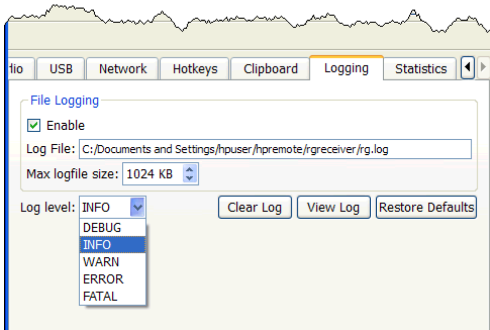
Figure 6-34 Options available under the Logging tab
