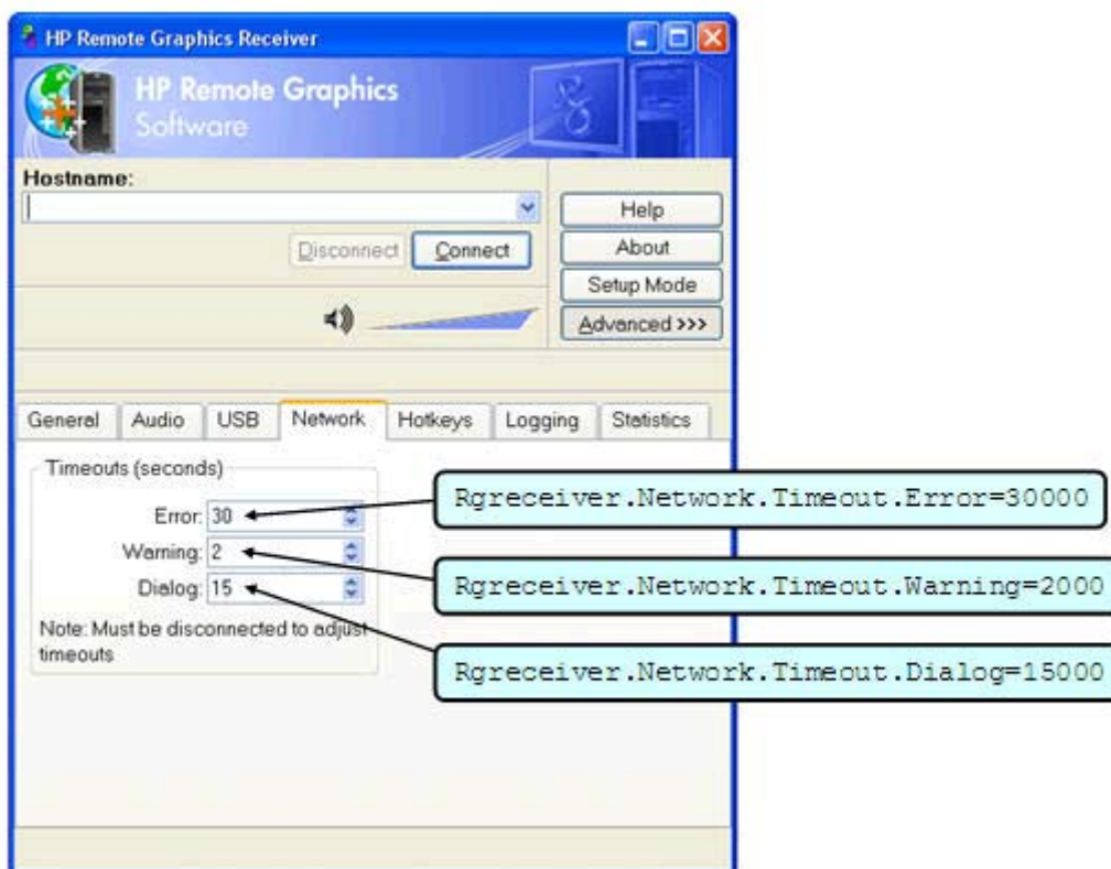
Figure 6-23 Receiver Control Panel
