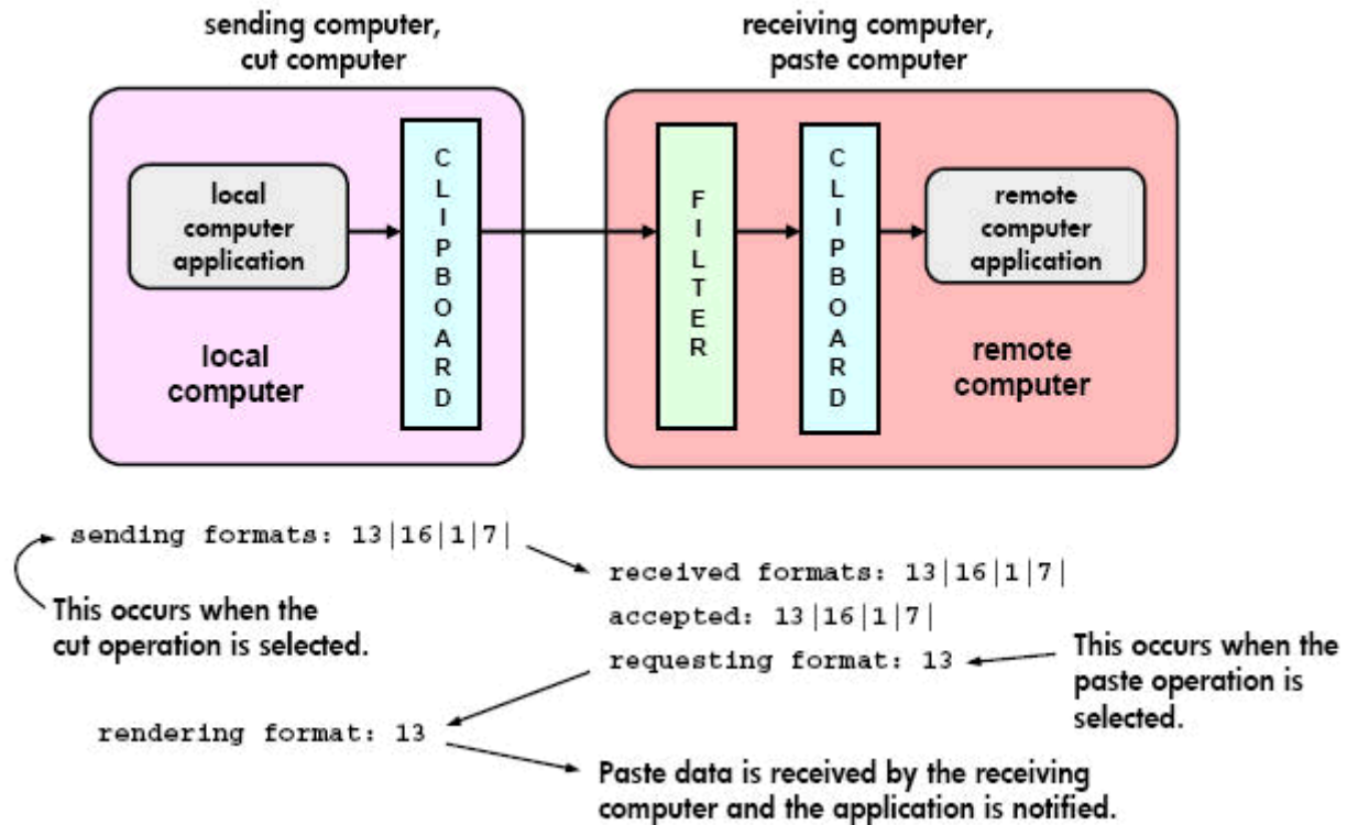
Figure 6-33 Remote Clipboard log entries for cut and paste
