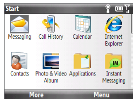
Start menu
