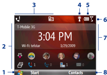
Home Screen
