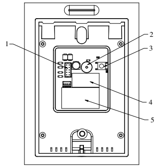
Figure 2-9 Rear View of DS-K1101 Series
