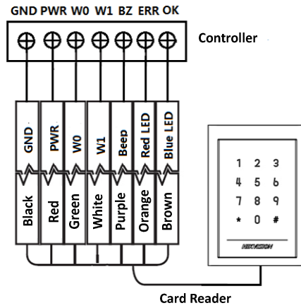
Figure 3-5 Wiring for Wiegand Communication Mode
