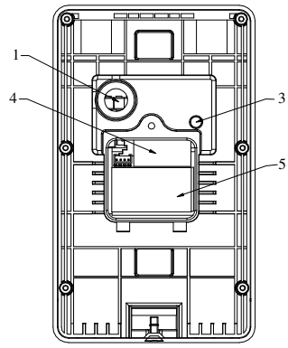
Figure 2-11 Rear View of DS-K1103 Series
