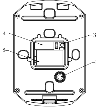
Figure 2-12 Rear View of DS-K1104 Series
