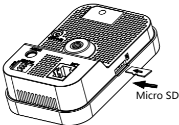
Figure 3-1 Install Micro SD Card
