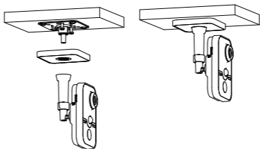
Figure 3-7 Install the Camera
