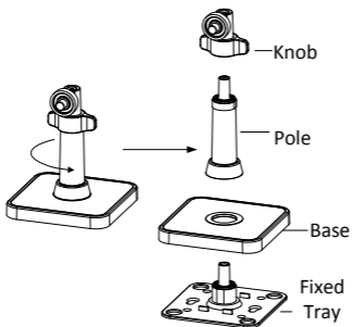
Figure 3-5 Disassemble the Bracket
