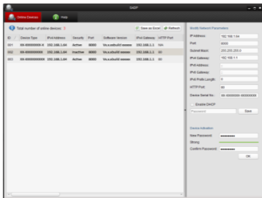
Figure 4-4 SADP Interface
