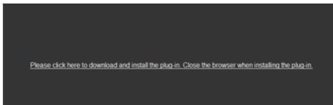
Figure 5-2 Download Plug-in
