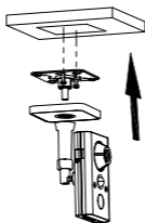
Figure 3-4 Ceiling Mounting
