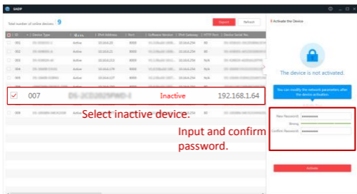
Figure 4-4 SADP Interface
