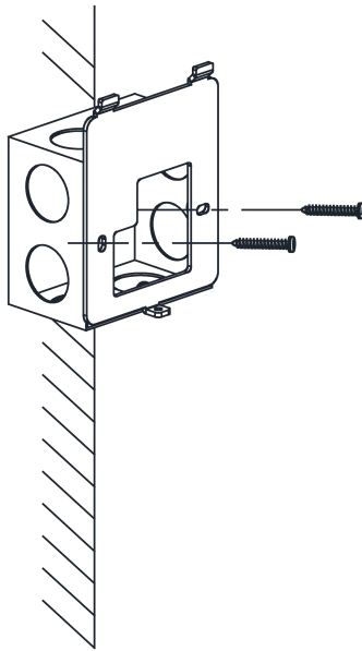
Figure 3-2 Install Mounting Plate
