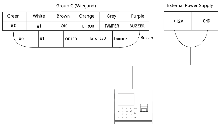
Figure 4-6 Wiring as Wiegand Card Reader
