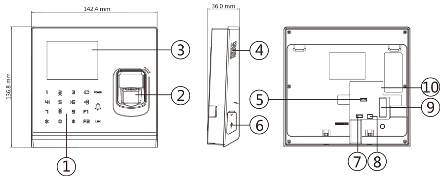
Figure 2-2 Diagram of Access Control Terminal Appearance (With Fingerprint Module)
