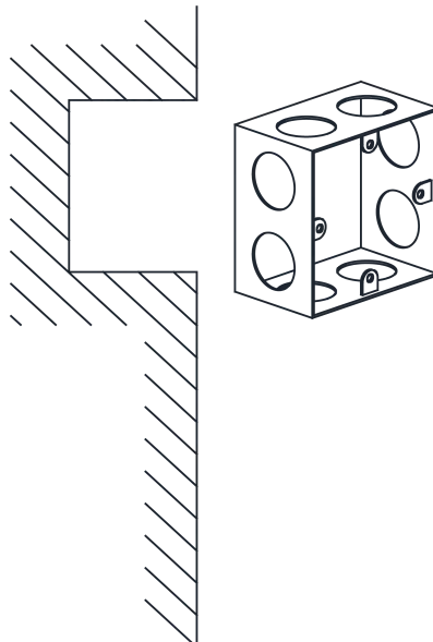
Figure 3-5 Install 86 Gang box
