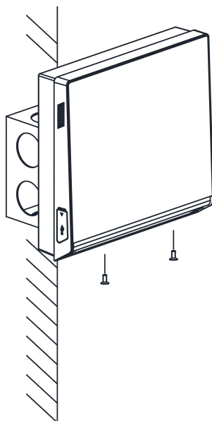
Figure 3-8 Tighten Screws
