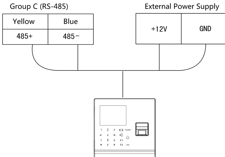
Figure 4-5 Wiring of RS-485 Output
