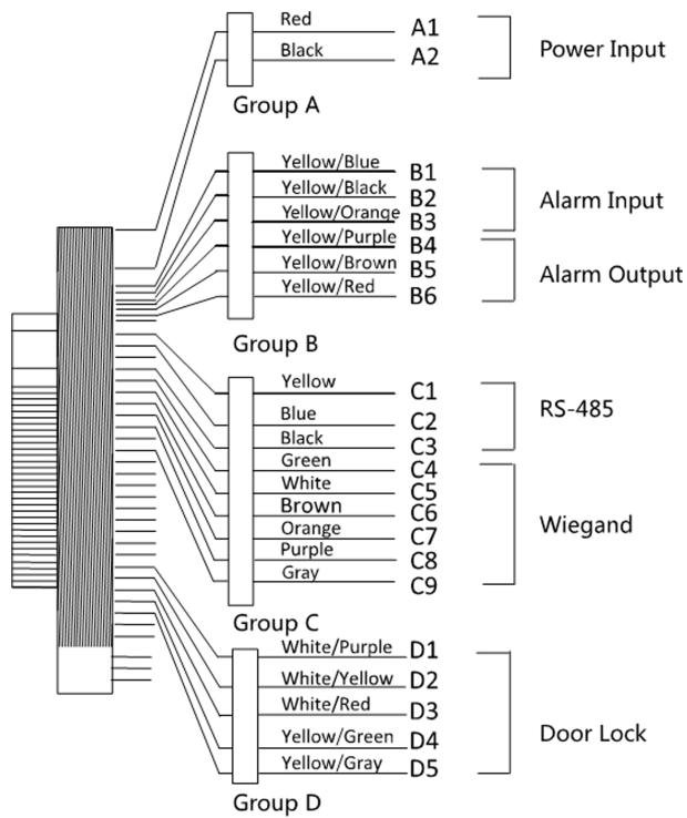
Figure 4-1 Terminal Diagram
