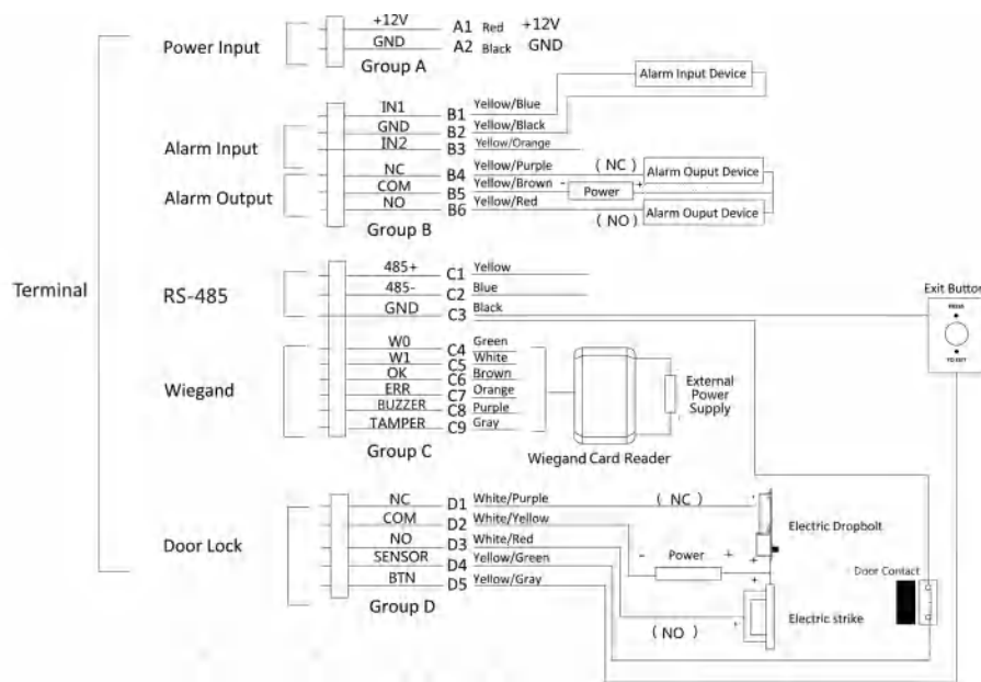
Figure 4-2 Wiring Overview
