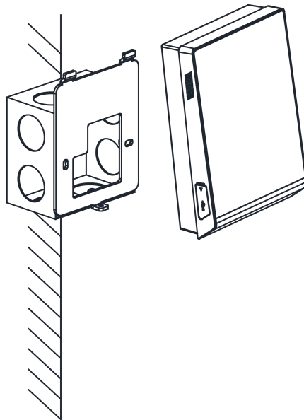
Figure 3-3 Buckle Terminal on Plate
