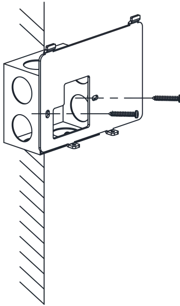
Figure 3-6 Install Mounting Plate
