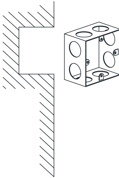
Figure 3-1 Install 86 Gang box
