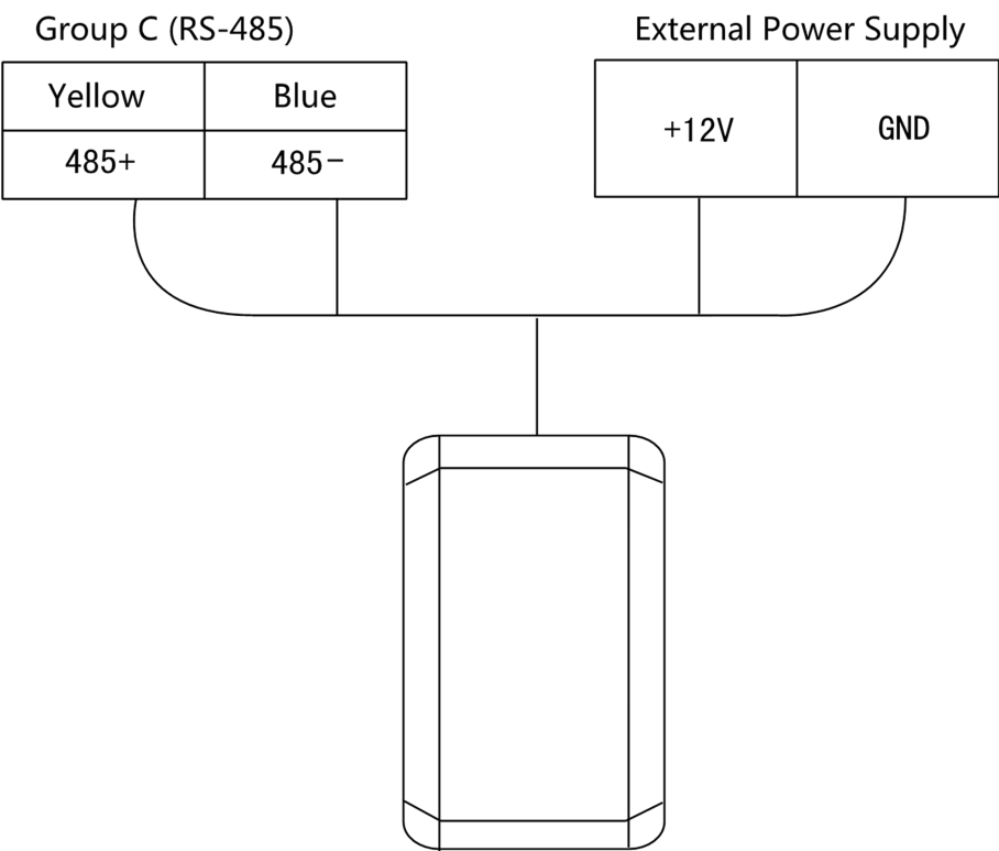
Figure 4-3 Wiring of External RS-485 Card Reader
