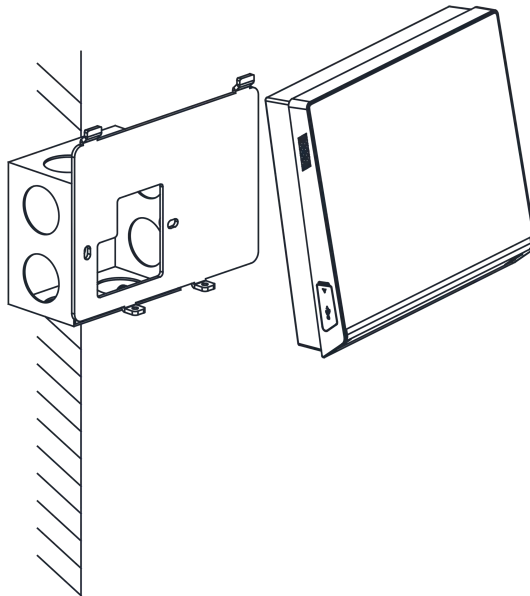
Figure 3-7 Buckle Terminal on Plate
