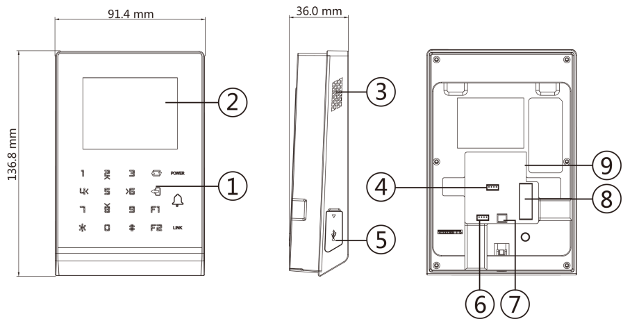
Figure 2-1 Diagram of Access Control Terminal Appearance (Without Fingerprint Module)
