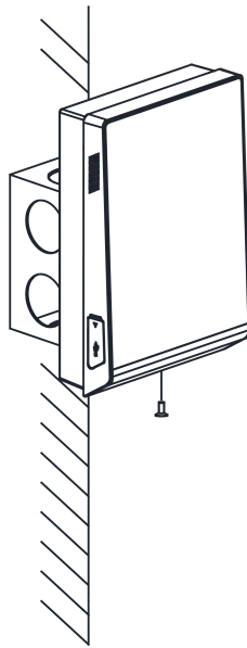
Figure 3-4 Tighten Screw
