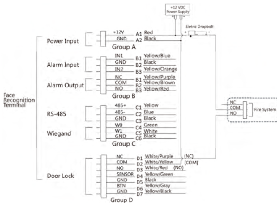
Figure 4-8 Wiring Device
