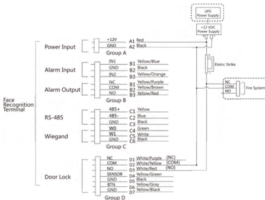
Figure 4-4 Device Wiring
