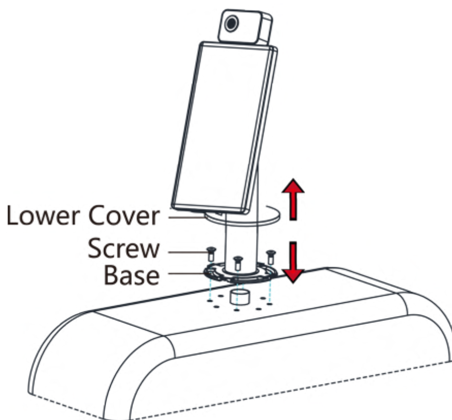
Figure 3-7 Secure Bracket and Turnstile
