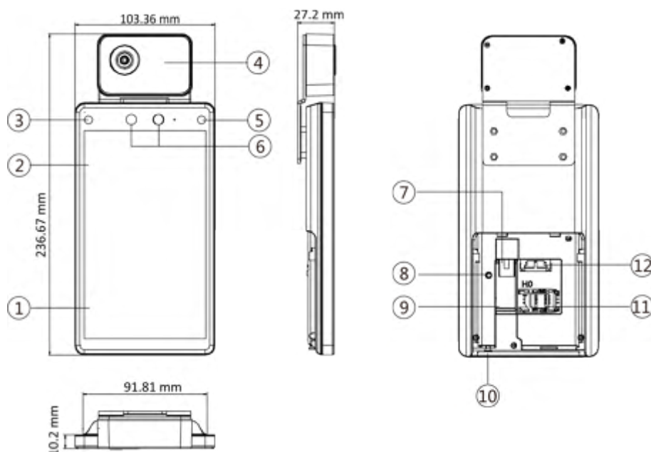
Figure 2-1 Face Recognition Terminal Diagram
