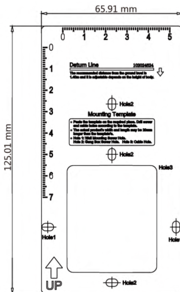
Figure 3-5 Mounting Template
