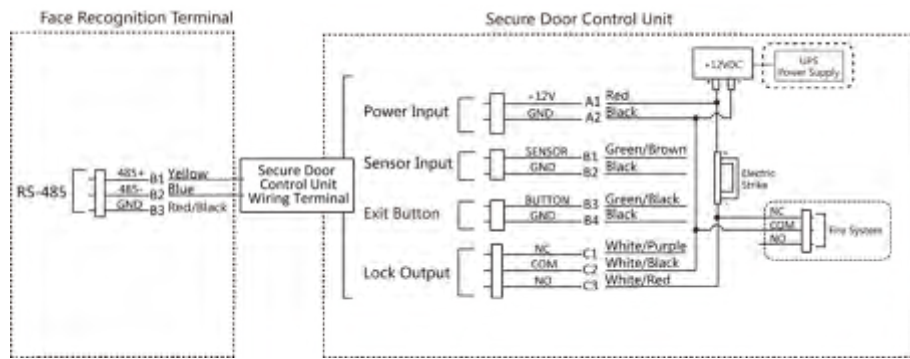
Figure 4-5 Wiring Diagram
