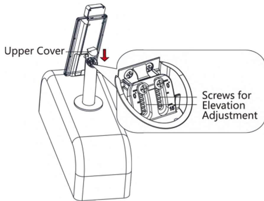
Figure 3-9 Adjust Elevation
