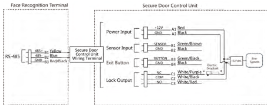
Figure 4-7 Wire Secure Door Control Unit
