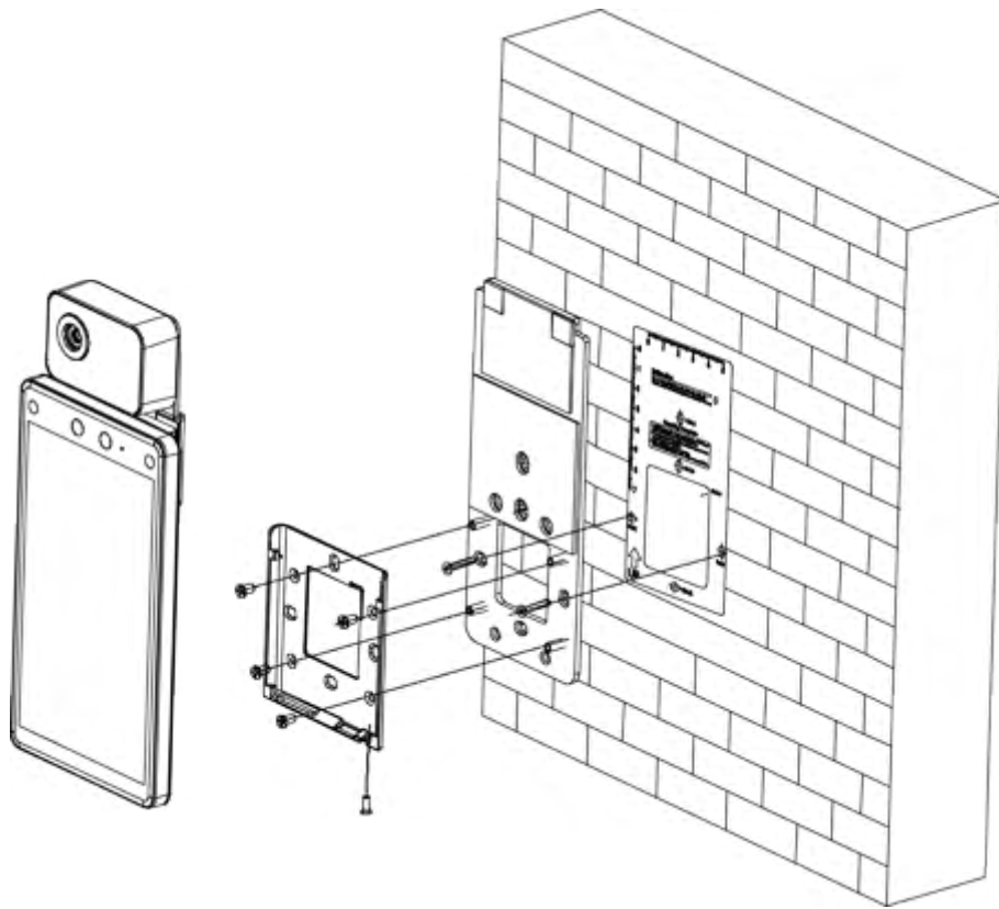
Figure 3-6 Install Device
