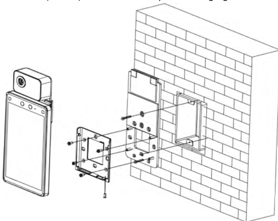
Figure 3-2 Install Device
