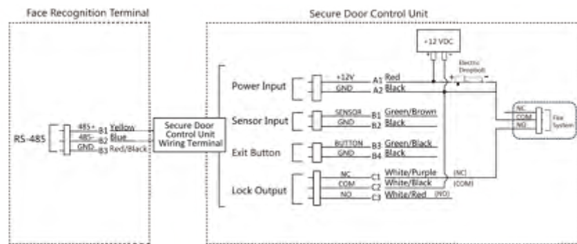
Figure 4-9 Wiring Secure Door Control Unit
