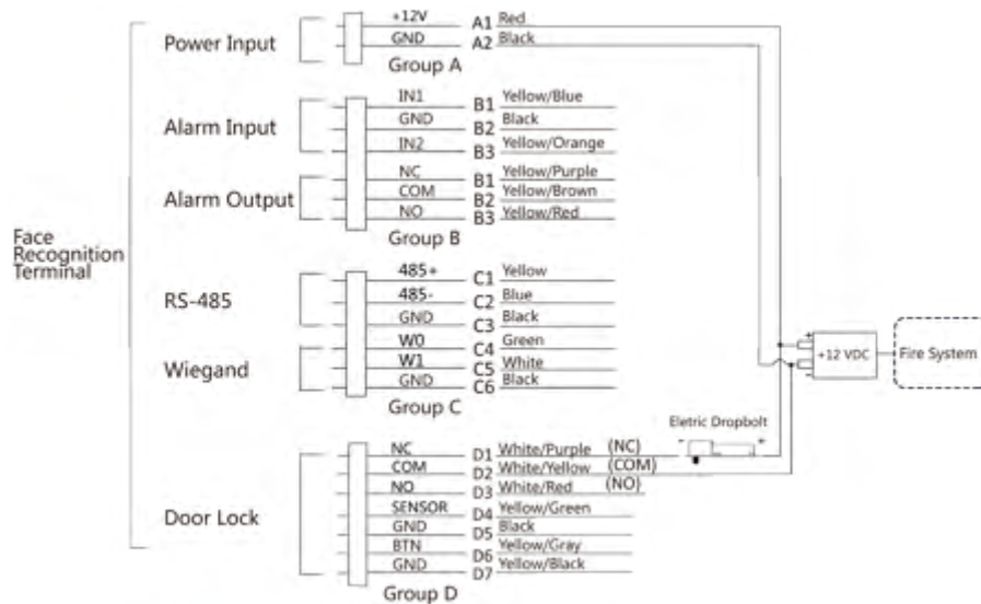
Figure 4-6 Wire Device
