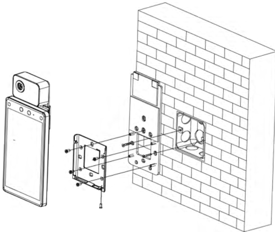
Figure 3-4 Install Device
