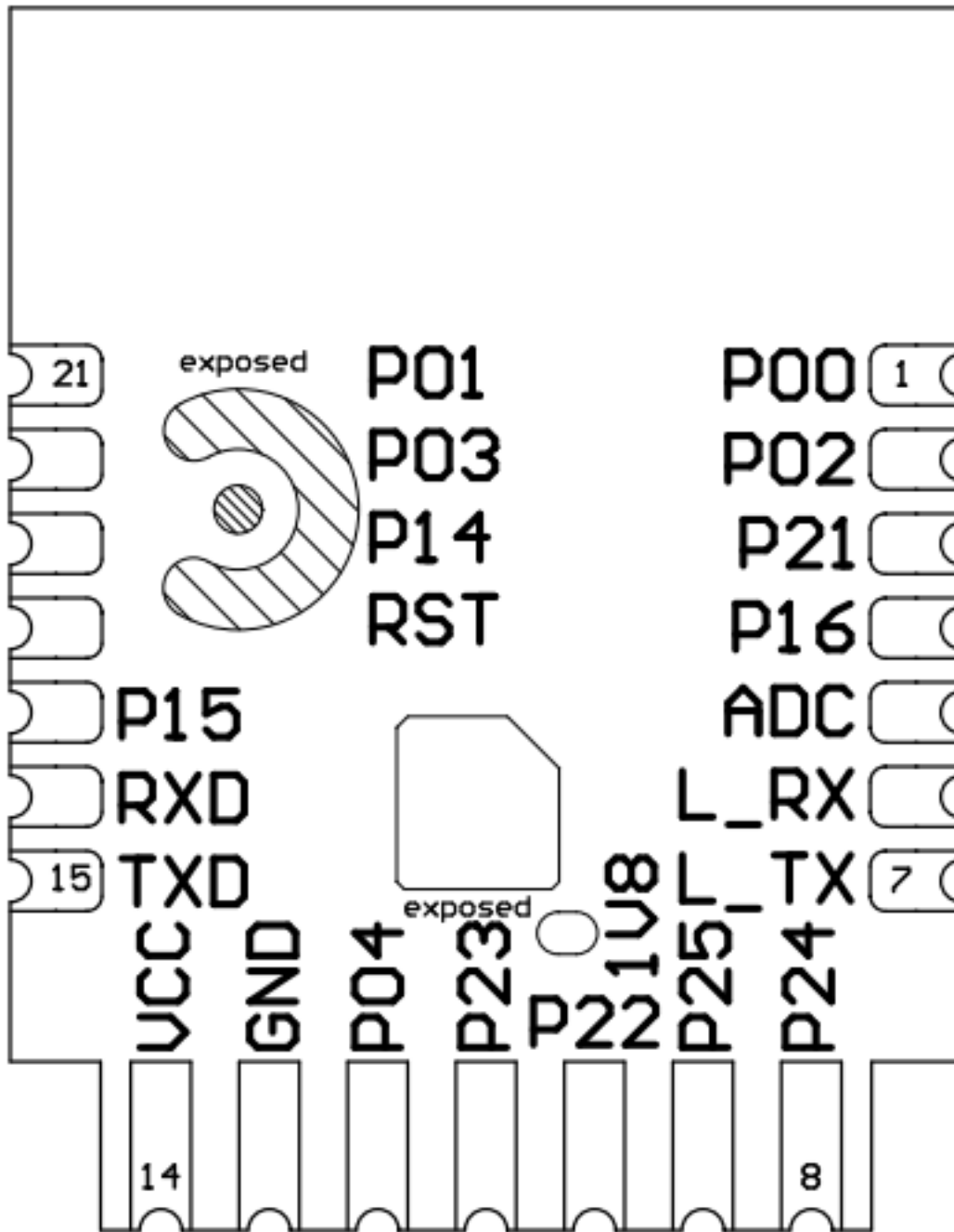
Bottom View
