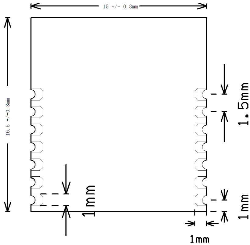
Figure 6-1 BT7L mechanical dimensions
