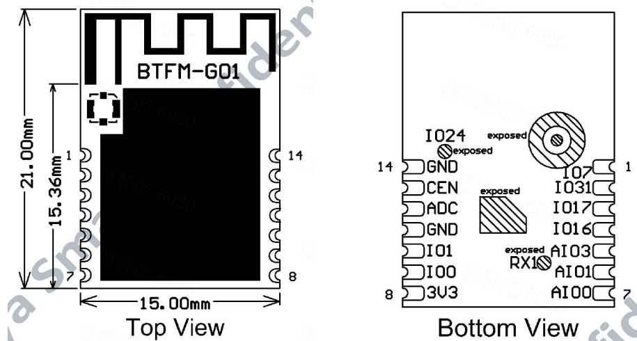
Figure 2-1 BTFM-G01 pins
