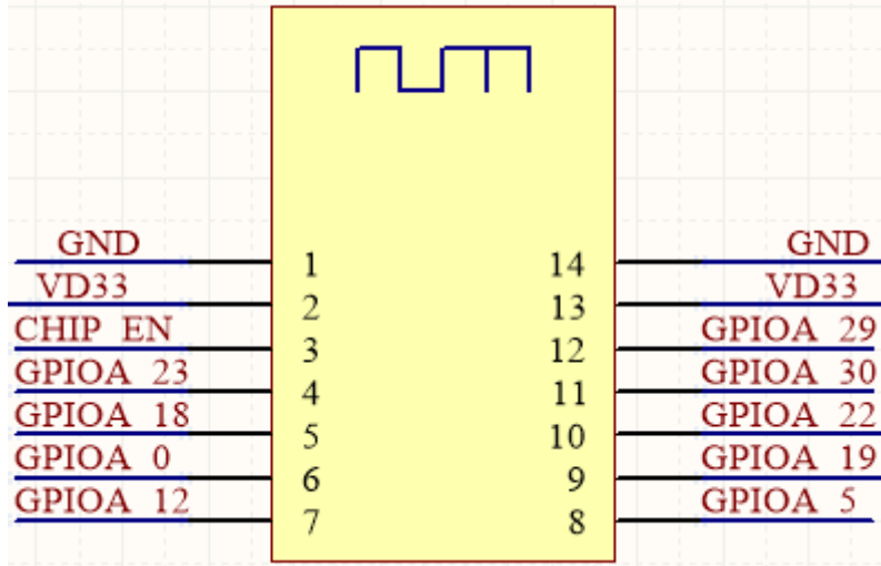
Figure 6.3. PCB schematic Drawing
