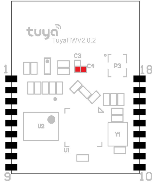
Figure 4. External Antenna configuration
