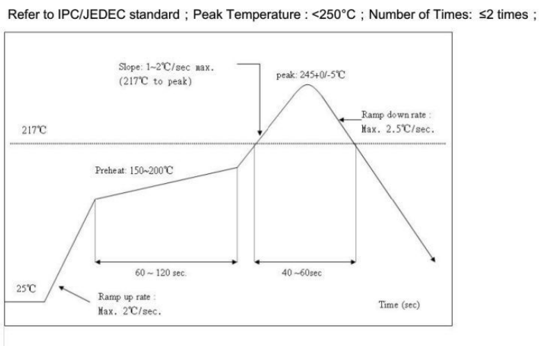
Figure 6.2. PCB Package Drawing Recommended furnace temperature curve
