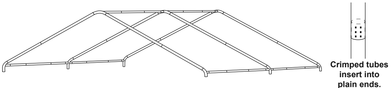
Figure B: Roof Assembly
