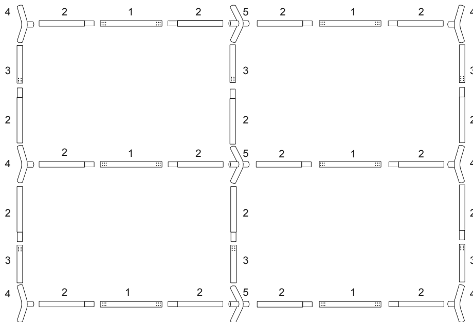
Figure A: Roof Layout
