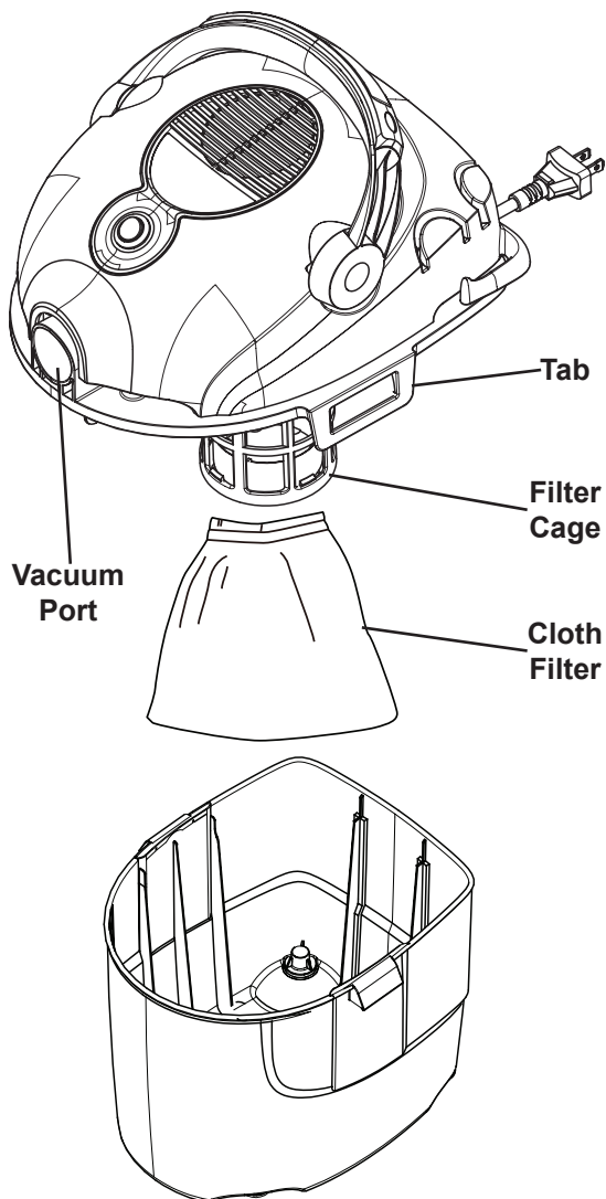
Figure A: Dry Vacuum Setup
