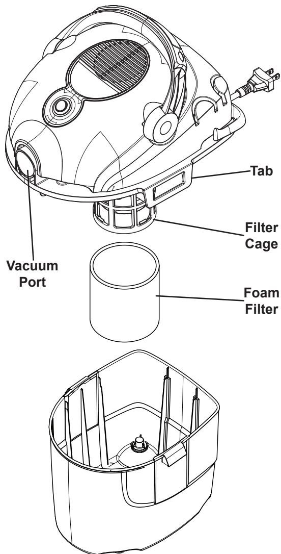
Figure B: Wet Vacuum Setup
